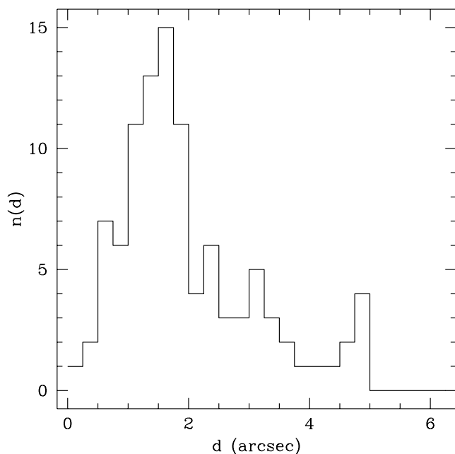
FIG. 3.—Distribution of positional distances between the centroids of the 3.6 \mu\text{m} sources and the Chandra sources. The distribution includes a slight systematic offset in declination, also apparent in Fig. 2, which, however, does not influence the source identification.
