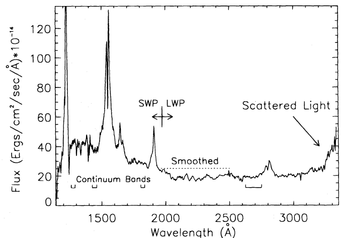
FIG. 1.—Averaged and combined SWP and LWP spectrum of NGC 4151 for the 1993 campaign. The 1975–2500 Å region has been smoothed with a 10 pixel ( \sim 15 Å) boxcar filter for display purposes.
