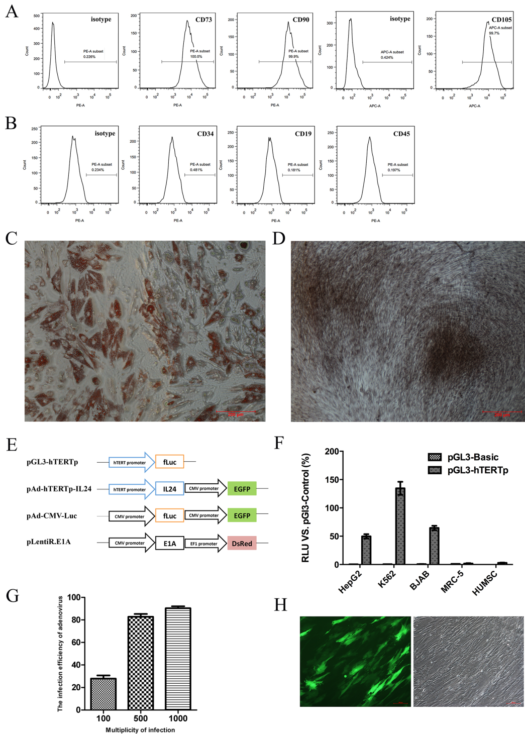
Figure 1: Identification of HUMSCs, the specific activity of hTERT promoter and adenoviral transfection efficiency.
