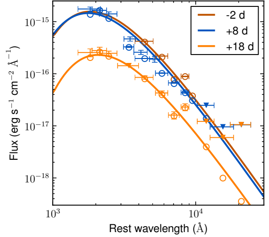
FIG. 4.— The SED of PS1-12sk from photometry at three epochs ( \text{MJD} = [56005, 56015, 56025] \pm 1.5 ). The circles show the linearly interpolated light curve value in each filter at each precise epoch, error bars show the flux and filter width for the measured NUV-NIR photometric points nearest to each epoch (only when within 1.5 days), and triangles show the nearest 3\sigma upper limit. The solid lines show the blackbody fit to the interpolated photometry. The NIR observations do not suggest a significant infrared excess for PS1-12sk within a few weeks of peak brightness.
