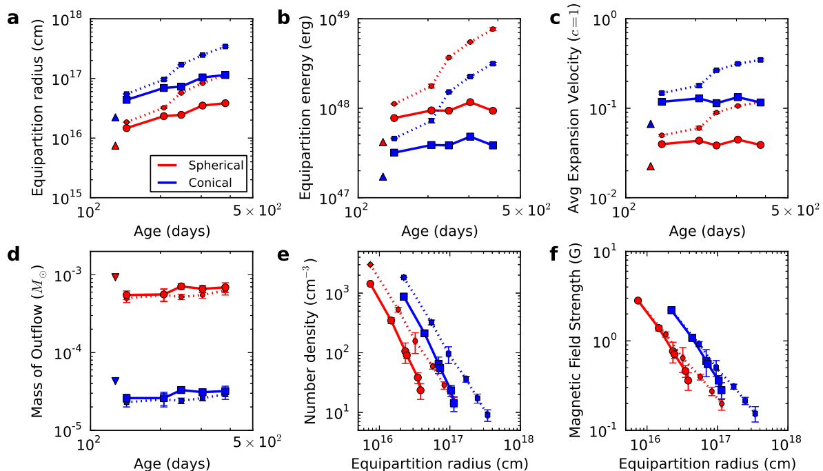
Figure 2. The temporal and radial dependencies of several physical quantities of the outflow inferred from synchrotron equipartition model fits to our radio observations. In each panel the dotted and solid lines mark the fits to the total radio flux densities (Figure 1, panel (a)) and transient flux density only (Figure 1, panel (b)), respectively. The red circles mark the results for a spherical outflow while the blue squares mark the results for a conical outflow with a covering fraction of 10%. We determine the radius of the emitting region as a function of time (a), the outflow kinetic energy as a function of time (b), the outflow expansion velocity as a function of time (c), the outflow mass as a function of time (d), the circumnuclear radial density profile (e), and the magnetic field radial profile (f). The errorbars on the data points in each panel correspond to 1 standard deviation and are computed using a Markov Chain Monte Carlo approach that takes into account the uncertainties in the synchrotron model parameters. The inferred quantities are summarized in Table 2.
