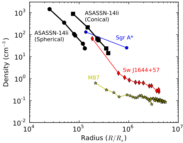
Figure 3. The radial density profile in the circumnuclear region of ASASSN-14li in comparison to other SMBHs. We infer a density profile of \rho(R) \propto R^{-2.5} on a scale of about 0.01 pc. For comparison, we show the density profiles for the Sgr A* (Baganoff et al. 2003), the nucleus of M87 (Russell et al. 2015), and the circumnuclear region of the \gamma -ray TDE Sw J1644+57 (Berger et al. 2012), which span the range of \rho(R) \propto R^{-3/2} to R^{-1} . To facilitate the comparison we scale the radii by the Schwarzschild radius of each SMBH ( R_s = 2GM_{\text{BH}}/c^2 , where M_{\text{BH}} is the black hole mass), using an estimate of M_{\text{BH}} \approx 10^6 M_{\odot} for ASASSN-14li (Holoien et al. 2016; Miller et al. 2015). We find that for the circumnuclear region of ASASSN-14li the density profile is steeper than previously seen in the other SMBH systems, but the density normalization is comparable.
