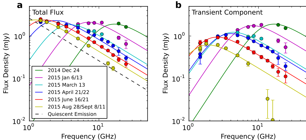
Figure 1. Radio observations of the TDE ASASSN-14li spanning December 2014 to September 2015. Filled circles mark the observed radio flux densities (in many cases, the errorbars, which correspond to 1 standard deviation, are smaller than the points; Table 1), while solid lines are best-fit models for synchrotron emission from a power-law distribution of electrons (Granot & Sari 2002; Barniol Duran et al. 2013), N(\gamma) \propto \gamma^{-3} for \gamma \geq \gamma_m (Section 4). (a) The total flux observed at each frequency. The dashed black line indicates a F_\nu \propto \nu^{-1} power law model for the underlying quiescent emission component, whose existence is implied by the archival radio detections. (b) Residual transient radio flux density obtained by subtracting the modeled quiescent emission component. These residual flux densities have a spectral shape characteristic of a synchrotron self-absorbed spectrum, with a spectral slope of F_\nu \propto \nu^{5/2} below the peak and F_\nu \propto \nu^{-1} above the peak. The evolution of the SED is typical of synchrotron emission from an expanding outflow. We note that our 2014 December 24 observations only weakly constrain the location of the spectral peak, so all parameters inferred for this epoch are considered to be lower limits.
