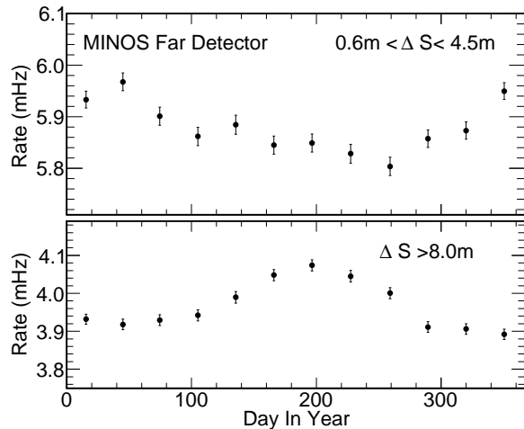
FIG. 5: The multiple-muon rate in the FD for events with \Delta S range A from 0.6 m to 4.5 m (top graph) and for events with \Delta S range C larger than 8 m (bottom) binned according to calendar month. The top figure shows a winter maximum. The bottom figure shows a summer maximum.
