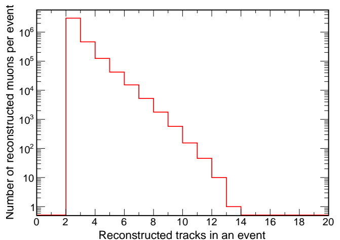
FIG. 2: The reconstructed muon multiplicity, for events containing more than one reconstructed track, in the Far Detector.
