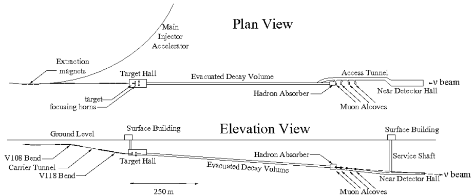
Figure 3: Plan and Elevation Views of the NuMI Beam Facility. The proton beam is directed onto a target, where subsequently the secondary pions and kaons are focused into an evacuated decay volume (later filled with helium) via magnetic horns. Ionization chambers at the end of the beam line measure the secondary hadron beam and tertiary muon beam.
