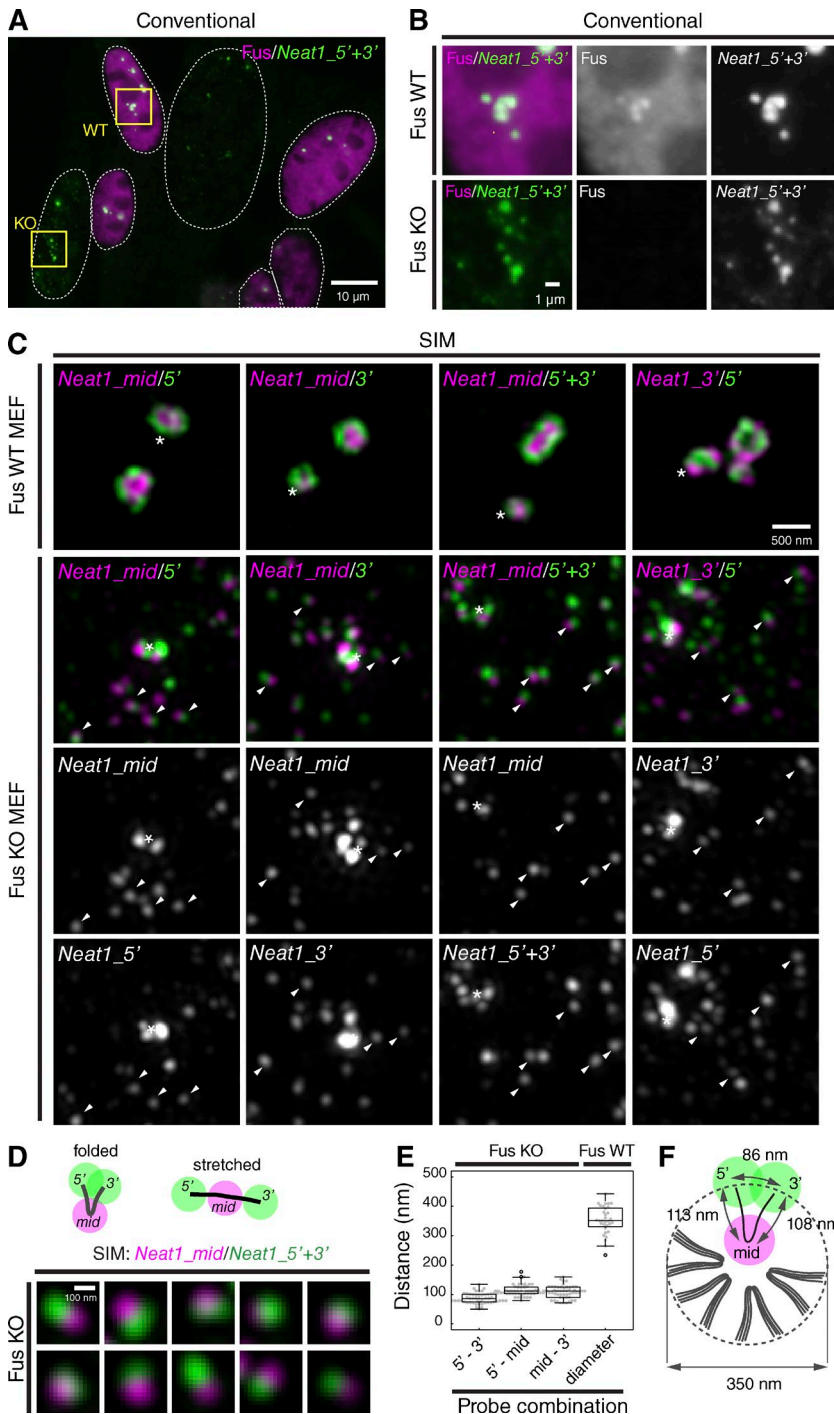
Figure 5. Fus is required for the assembly of the core-shell structure of paraspeckles. (A) Simultaneous detection of Fus and Neat1 in a mixture of MEFs prepared from WT and Fus KO mice using a conventional epifluorescence microscope (Conventional). Yellow boxes indicate the areas shown at a higher magnification in B. Note that Neat1 forms discrete nuclear body-like structures in Fus KO MEFs. (B) Higher magnification images shown in yellow boxes in A. (C) SIM observation of Neat1 in WT and Fus KO MEFs using the region-specific probes. Note that the characteristic core-shell structure was not observed in the Fus KO MEFs. Asterisks indicate the position of the putative transcription sites detected with the Neat1 tail probe. Arrowheads indicate Neat1 primary units containing both of the detected regions of Neat1 . (D) Models of the Neat1 primary unit and higher magnification images of FISH signals obtained with the Neat1_5'+3' probe in Fus KO MEFs. Note the close association of the two signals. (E) Measurement of the distance between the two different regions of Neat1 in Fus KO MEFs. Note that the distance between the 5' and 3' region of Neat1 is shorter than the distance between the 5' and the middle or the middle and the 3' regions of Neat1 . The median is indicated with a horizontal line in a box that represents the first and third quartiles. Outliers are indicated as circles, and the maximum and minimum are indicated at the end of the whiskers. Each dot represents each signal of Neat1 particle. (F) A model of the organization of Neat1 in paraspeckle spheres. Bars: (A) 10 \mu m; (B) 1 \mu m; (C) 500 nm; (D) 100 nm.
