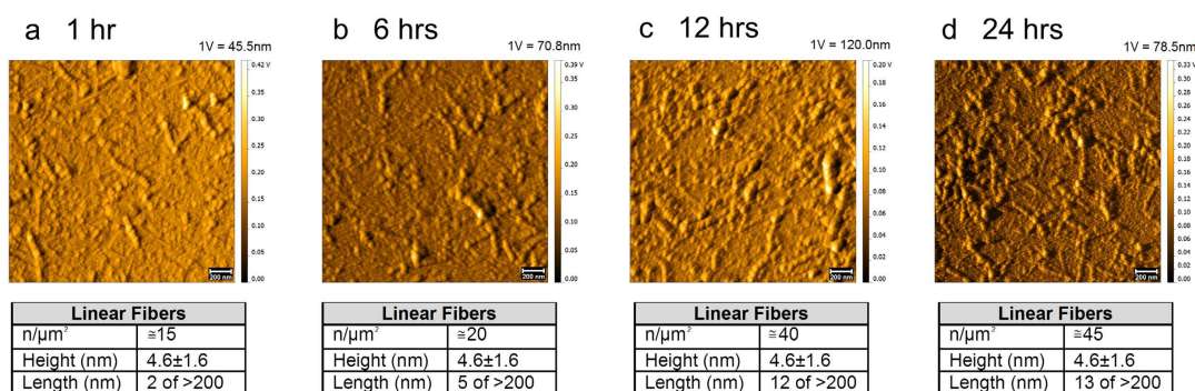
Figure 4. Fibril adsorption on primary mica surface. PAO were fibrillated and adsorbed on primary (Iry) mica and followed up to 24 hrs. Images show progressive growth of the number and size of the fibrils. Scale bars: 200 nm. PAO were fibrillated as reported in the Methods section. TM topography images show progressive growth of the number and size of the fibrils. At all the investigated times, the length of the fibril varies from 80 to 700 nm. The number and size of the structures are indicated in the table under each experimental time point. The amplitude scale is in Volt; we indicated the height (nm) corresponding to 1 Volt.
