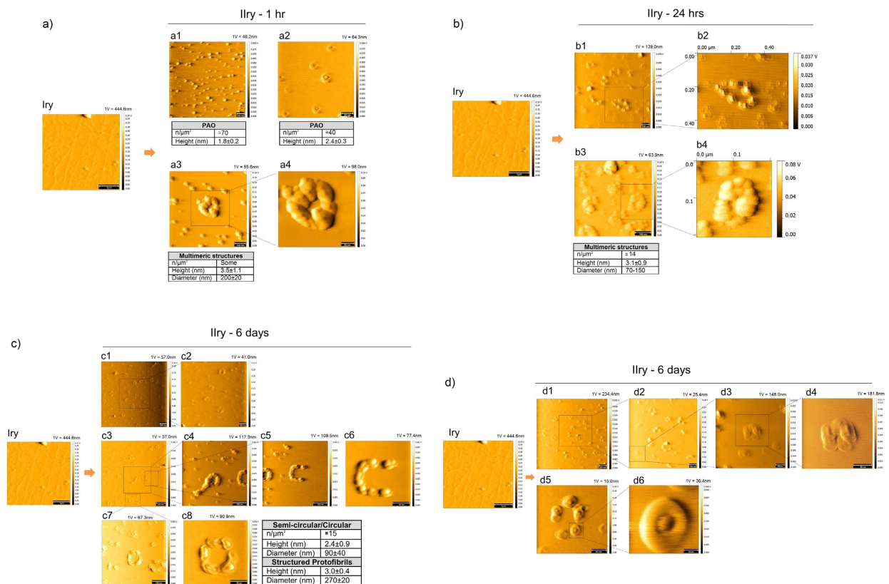
Figure 5. PAO budding and migration. Fibrils were adsorbed on primary (Iry) mica surface (scale bar 1 \mu\text{m} ). An empty secondary (IIry) mica was placed in contact with the primary mica and followed up to 6 days. Contact solution: 10 mM PBS at pH 7.4, T = 25^\circ\text{C} . A TM representative topography image of a pristine primary coated with fibrils is shown as primary (Iry). (a) Numerous PAO are adsorbed on the secondary mica after 1 hr of contact (scale bars: 50 nm (a2,a4) and 100 nm (a1,a3)). At this time transitional structures (a2) and scarce annular protofibrils (a3–a4) are adsorbed on the IIry. (b) More complex multimeric structures (MS) appear after 24 hrs (scale bars: 100 nm). The inserts b2 and b4 were magnified with the software therefore do not have the scale bar within the figure. (c,d) semi circular, circular (c1–c8) and more structured protofibrils (c4) and transitional structures (d5,d6), appear after 6 days (scale bars: 10 nm (d6), 50 nm (c6,c8,d3–d5), 100 nm (c2,c4,c5,c7,d2), and 200 nm (c1,c3,d1)). The number and size of the structures are indicated in the table under each experimental time point. The amplitude scale is in Volt; we indicated the height (nm) corresponding to 1 Volt.
