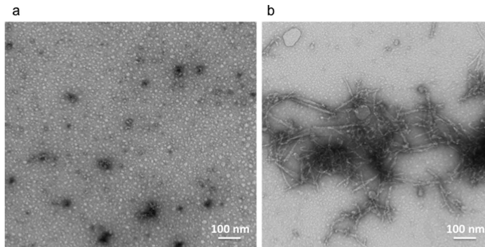
Figure 1. PAO and amyloid fibers transmission electron micrographs of: (a) the PAO synthesized in-vitro ; (b) the amyloid fibers formed after addition of a 5 v/v% hexane solution to the PAO in suspension.
