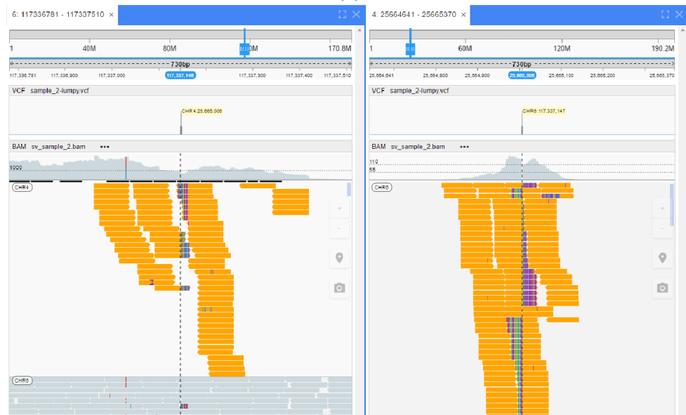
Figure 5 ROS1-SLC34A2 interchromosomal translocation fusion. (A) shows the effect of the fusion and (B) the read evidence for the event at both breakpoints.
