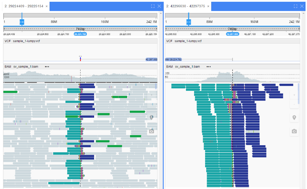
Figure 6 EML4-ALK inversion fusion. (A) shows the effect of the fusion and (B) the read evidence for the event at both breakpoints.
