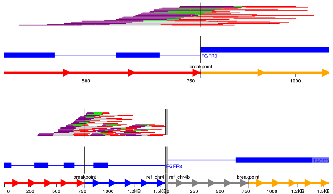
Figure 3 Sviz output for the FGFR3-TACC3 fusion (tandem duplication) in the RT4 cell line. Read evidence is shown for both how the last intron of FGFR3 is fused to an exon of TACC3 as well as for the reference alleles.
