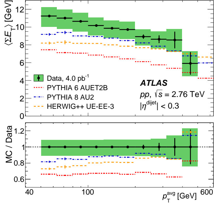
Figure 3: Measured \langle \Sigma E_T \rangle in hard-scatter pp collisions, shown as a function of p_T^{\text{avg}} for |\eta^{\text{dijet}}| < 0.3 and in comparison with the predictions of three MC event generators. The vertical shaded bands represent total systematic and statistical uncertainties in the data in quadrature while the vertical bars represent statistical uncertainties only. The bottom panel shows the ratio of the predictions of the three MC generators to the data.
