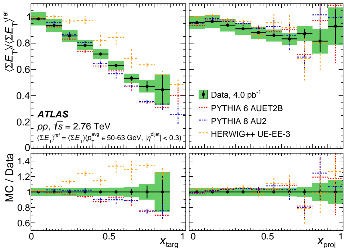
Figure 5: Measured ratio \langle \sum E_T \rangle / \langle \sum E_T \rangle^{\text{ref}} in hard-scatter pp collisions, shown as a function of x_{\text{targ}} (left) and x_{\text{proj}} (right). The vertical shaded bands represent total systematic and statistical uncertainties in the data in quadrature while the vertical bars represent statistical uncertainties only. The bottom panel shows the ratio of the predictions of three MC event generators to the data.
