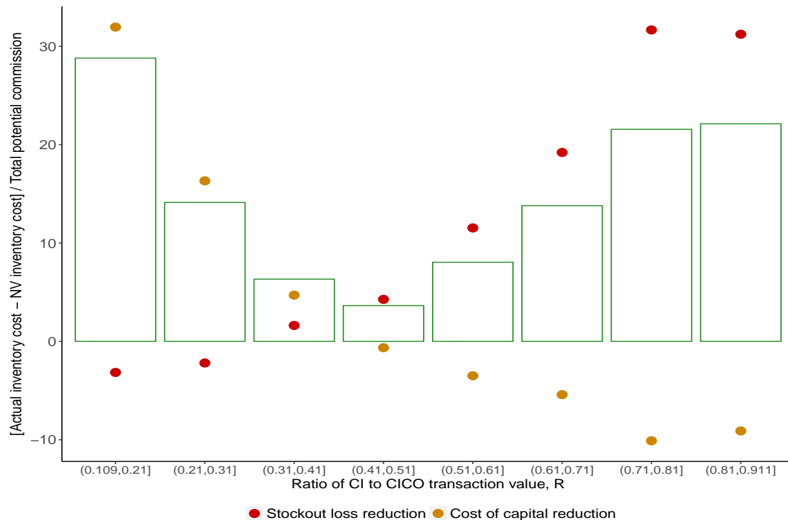
Figure 6 Performance differential between actual agent decisions and newsvendor heuristic recommendations by level of agent CICO balance
