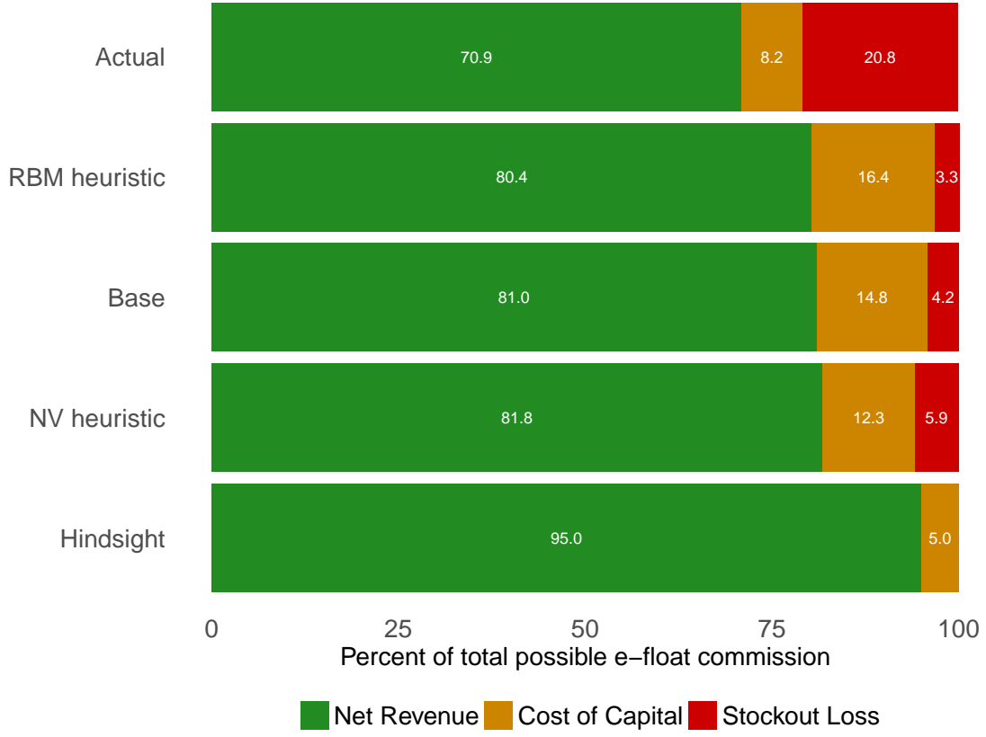
Figure A.1 Performance evaluation: aggregate net e-float revenue for actual agent decisions, RBM heuristic, base model, newsvendor heuristic, and hindsight recommendations over 180 days
