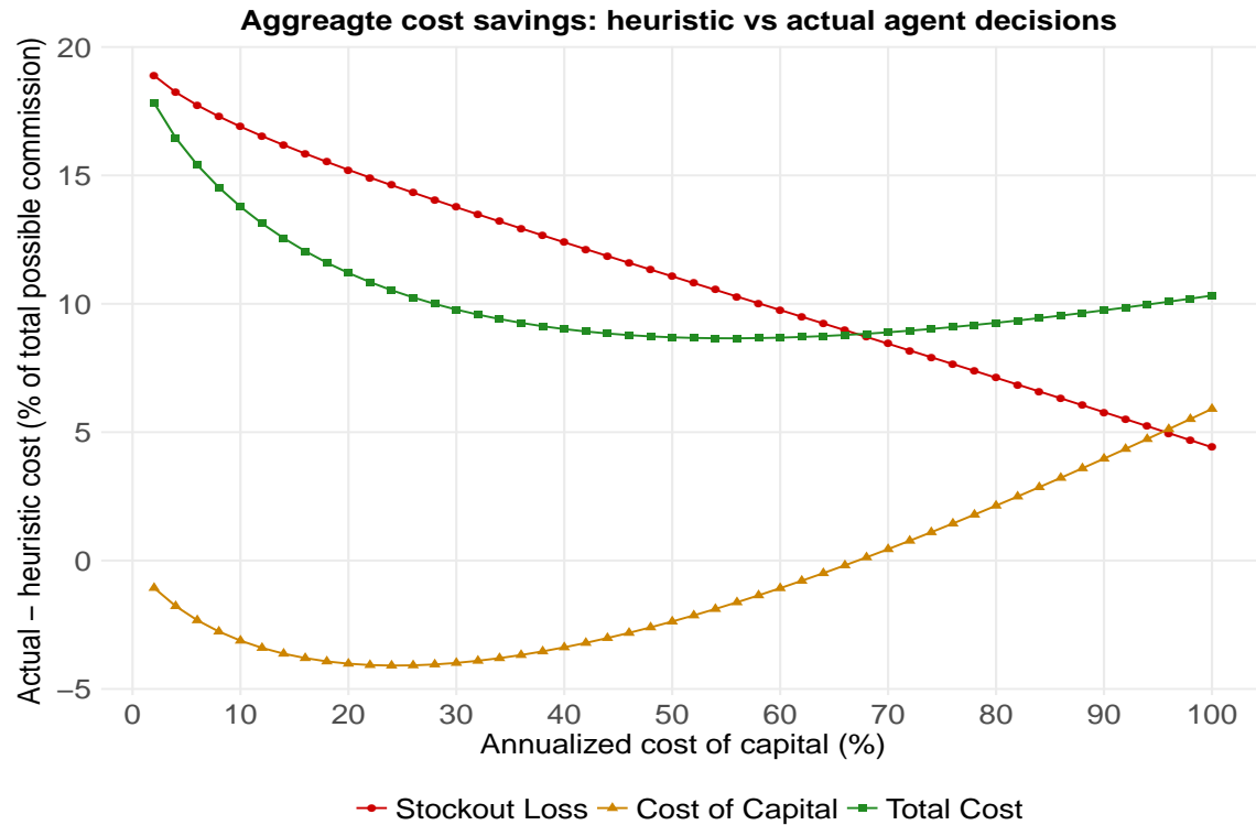
Figure 5 Cost savings sensitivity as a function of cost of capital: performance differential between actual agent decisions and newsvendor heuristic recommendations
