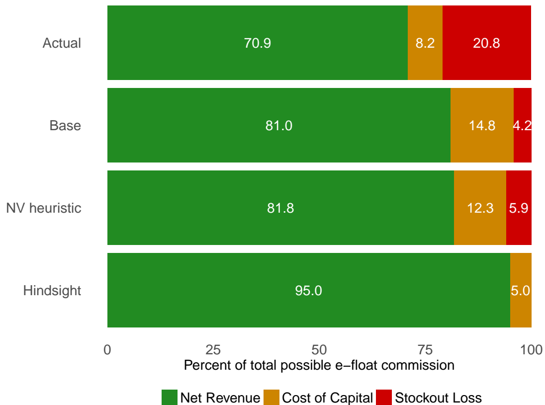
Figure 3 Performance evaluation: aggregate net e-float revenue for actual agent decisions, base model, newsvendor heuristic, and hindsight recommendations over 180 days
