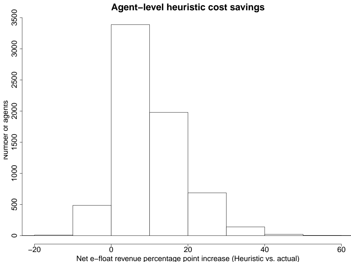
Figure 4 Agent-level e-float cost savings as a percent of total possible commission (heuristic vs. actual)
