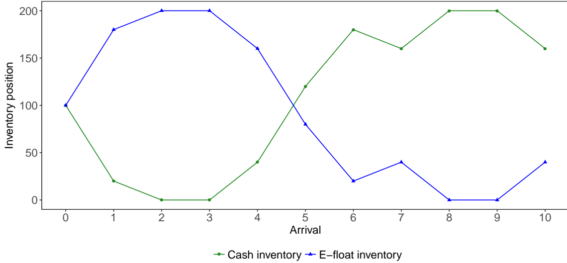
Figure 2 An illustrative example of agent inventory balances of cash and e-float
