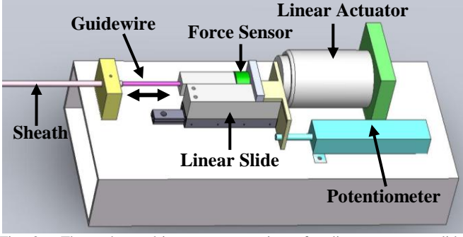
Fig. 2. The catheter drive system consists of a linear actuator, slide, potentiometer, and a force sensor to evaluate the friction on the catheter guidewire. The system servos the guidewire inside the fixed sheath.
