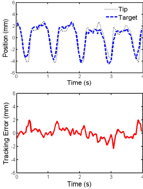
Fig. 17. Top: Trajectory of the catheter tip and the mitral valve annulus found by manual segmentation. Bottom: The catheter trajectory tracking error. RMS tracking error was 0.77 mm.
