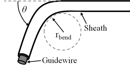
Fig. 5. The catheter sheath configurations used to evaluate the friction and backlash performance limitations.
