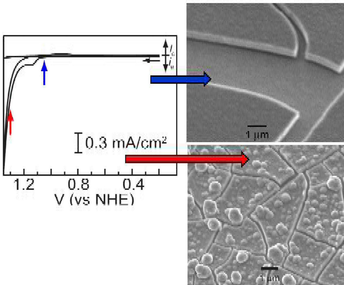
Figure 12. Cyclic voltammogram of a aqueous solution containing 1 mM Co 2+ and 0.1 M Pi electrolyte. SEM images are shown of catalyst films that form holding the electrode at the indicated pre-catalytic and catalytic potential.
