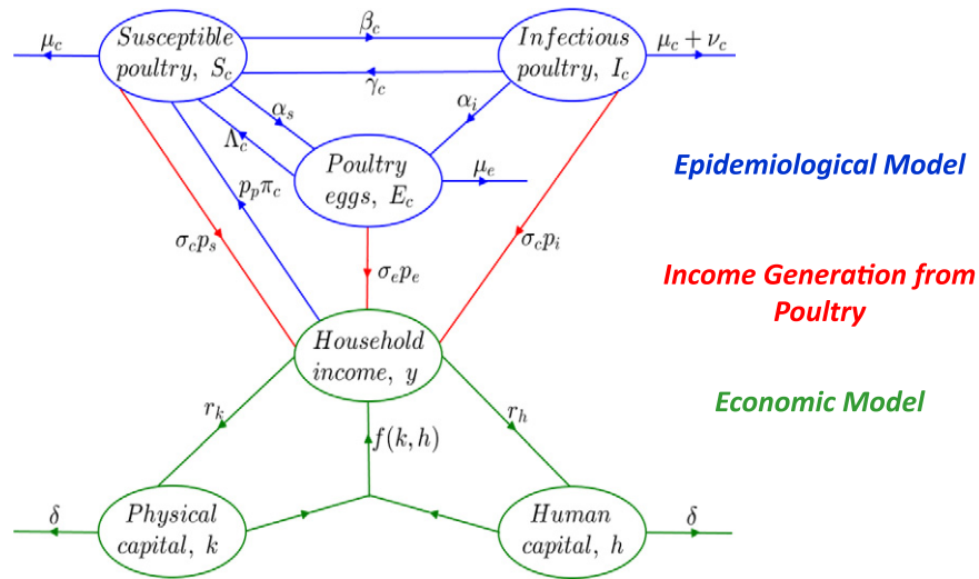
Fig. 1. Schematic of the coupled model. Blue ellipses denote poultry compartments, while blue lines denote transition rates between poultry compartments such as disease transmission rate, \beta_c , recovery rate, \gamma_c , natural mortality rate, \mu_c , disease-induced mortality rate, \nu_c , birth rate, \Lambda_c , egg-laying rates by healthy and unhealthy poultry, \alpha_s and \alpha_i , egg loss at rate, \mu_e ; and the use of income to purchase poultry, p_p \pi_c . Green ellipses denote economic model classes, while green lines denote the generation of income from physical and human capital, f(k, h) , and the reinvestment of a portion of income into these forms of capital at rates r_k and r_h . Red lines denote the generation of income through the sales and consumption of susceptible poultry, \sigma_c p_s , infectious poultry, \sigma_c p_i , and eggs, \sigma_e p_e .
