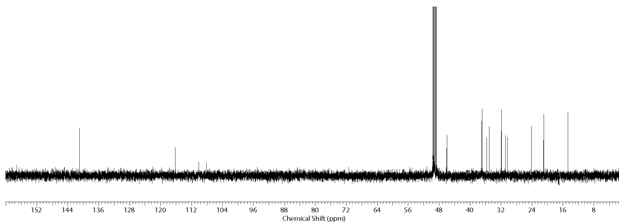
Figure 2.3: 13 C-NMR spectrum of cylindrocyclophane F in d 4 -methanol (125 MHz).
