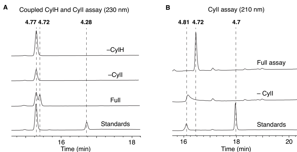
Figure 4.15: HPLC analysis of the CylH and CylII assays using chlorinated substrates. A) Coupled assay with the final module of the type I PKS CylH and the type III PKS CylII using 4.77 . B) Assay with CylII using 4.81 . Standard contains substrate 4.81 and cylindrocyclophane 4.7 (shift in retention time is observed due to an addition of a guard column).
