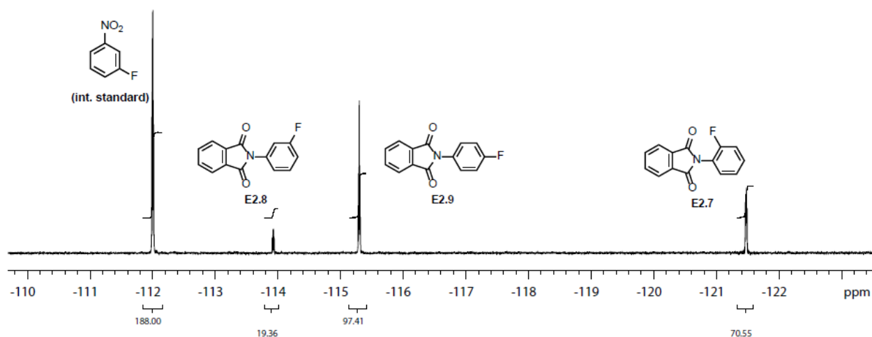
Figure E2.11. 19 F NMR analysis of product mixture of phthalimidyl radical substitution (CD 3 CN, 23 °C)
