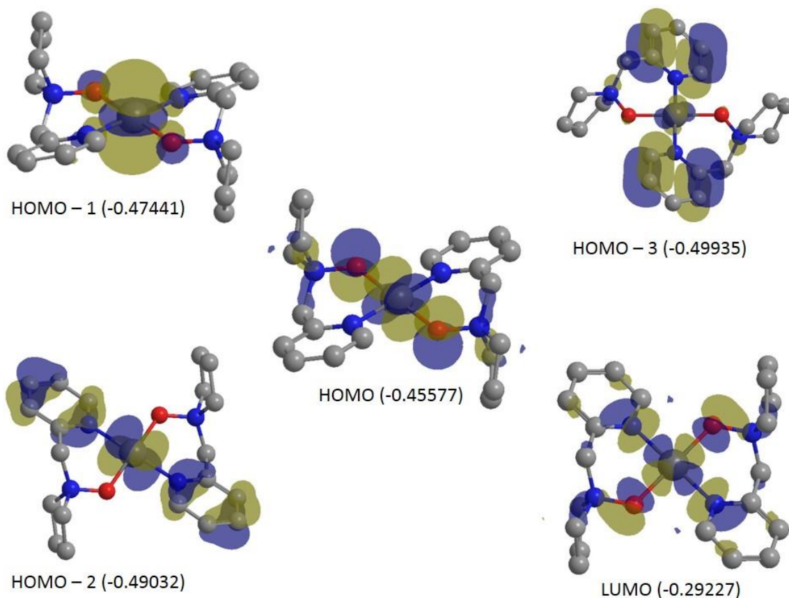
Figure E1.22. Valence orbitals and LUMO of 1.1 with energies in Hartrees
