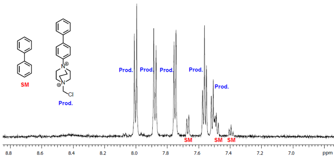
Figure E2.17. ^1\text{H} NMR of biphenyl TEDAylation reaction mixture ( \text{CD}_3\text{CN} , 23\text{ }^\circ\text{C} )
