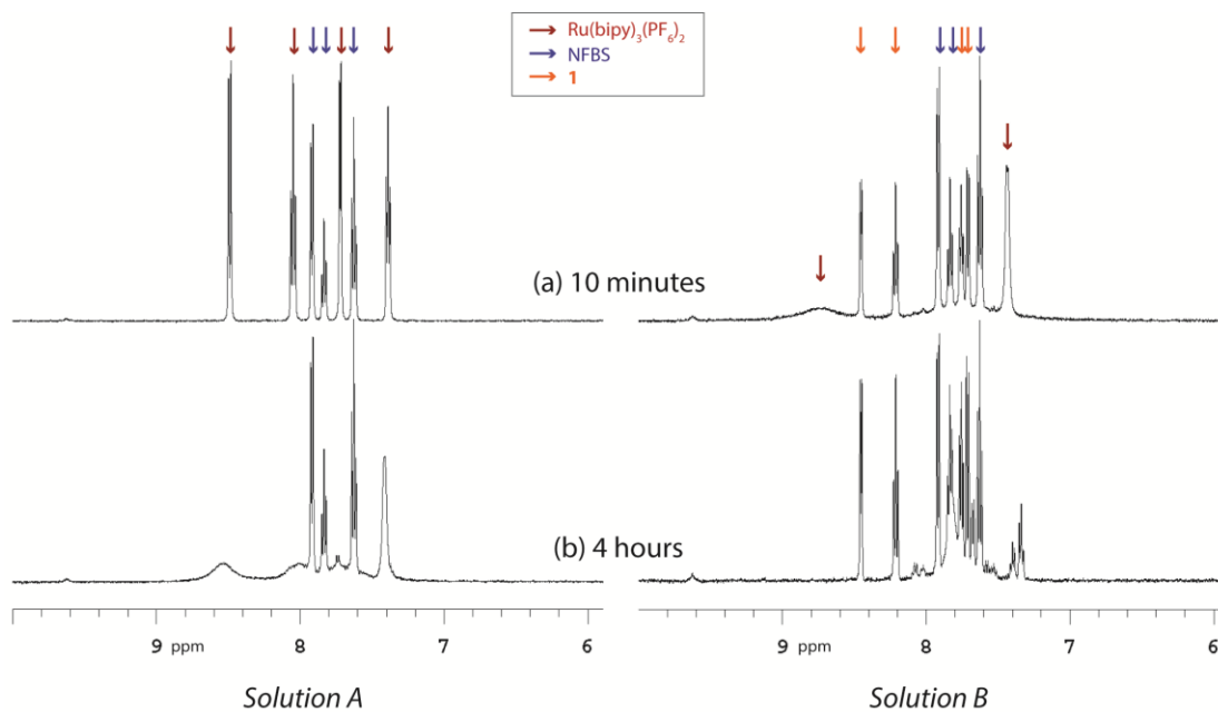
Figure E1.17. ^1\text{H} NMR spectra of Solution A (left) and Solution B (right) after 10 minutes (a, top) and 4 hours (b, bottom)
