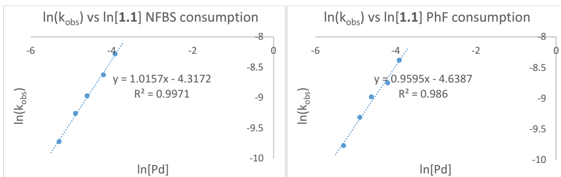
Figure E1.14. Determination of order in 1.1
