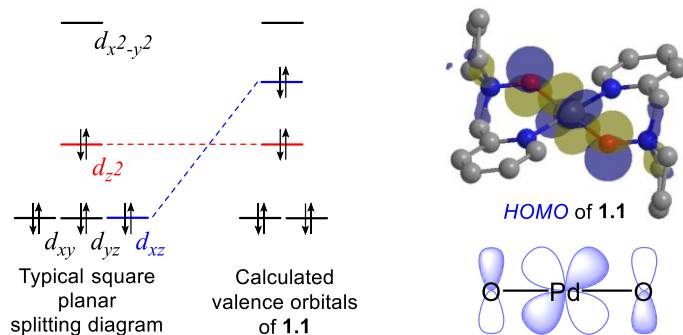
Figure 1.4. Valence orbital diagram of 1.1
