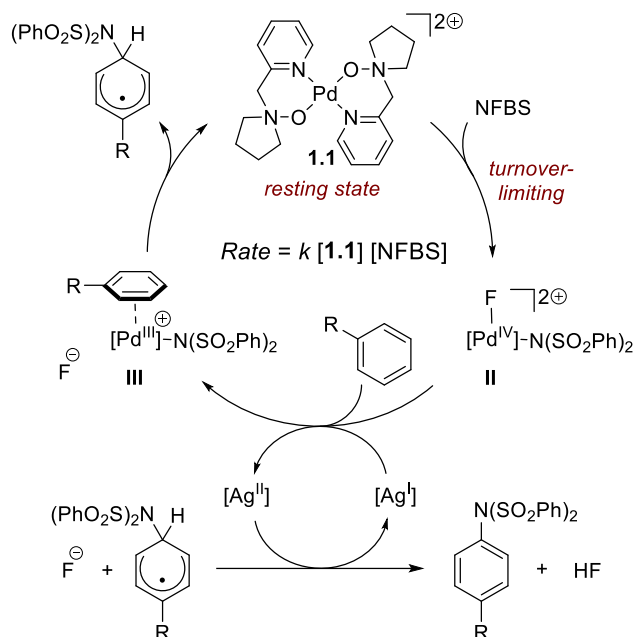
Figure 1.2. Proposed catalytic cycle
