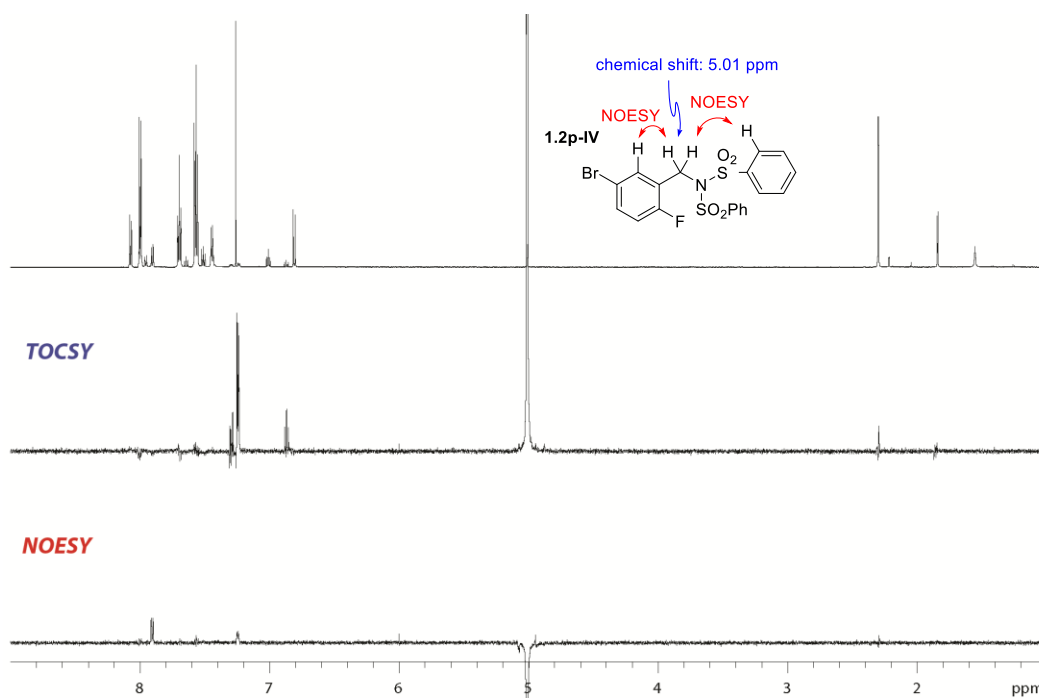
Figure E1.5. Structural assignment of 1.2p-IV by 1-D TOCSY and NOESY NMR ( \text{CDCl}_3 , 23 °C)
