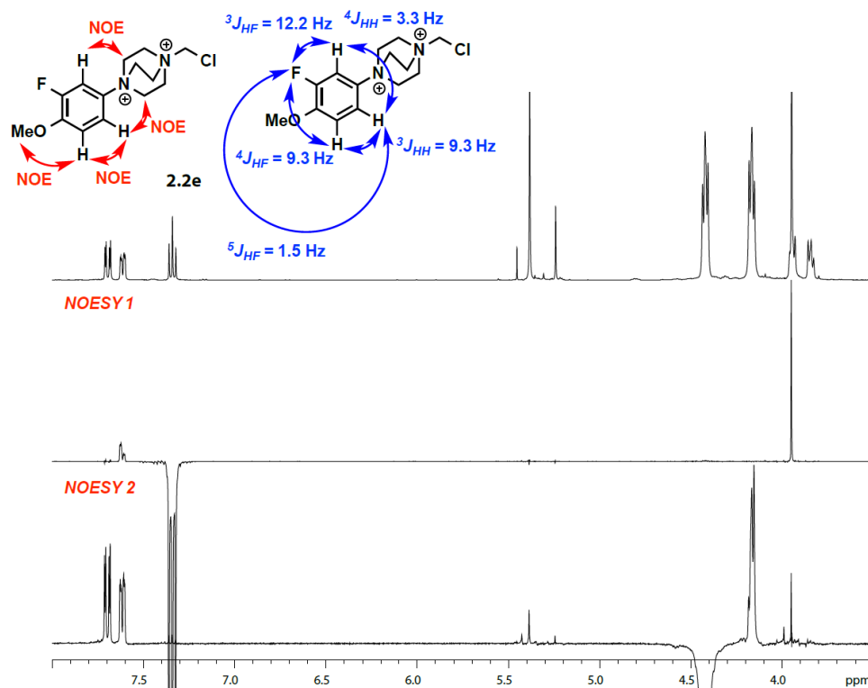
Figure E2.6. Assignment of 2.2e by 1-D NOESY NMR
