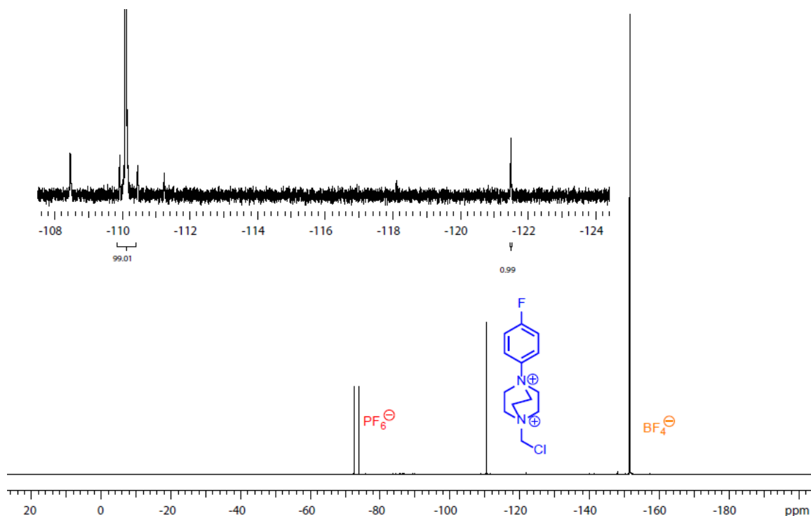
Figure E2.2. 19 F NMR evaluation of positional selectivity
