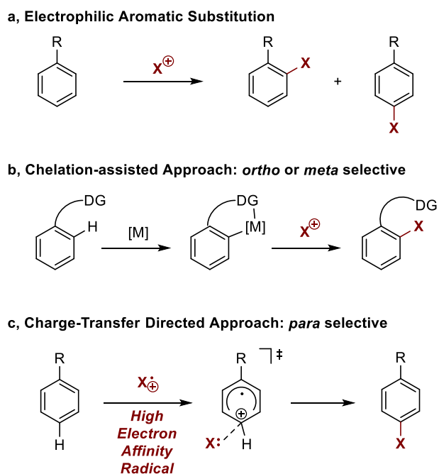
Figure 2.1. Selective C–H functionalization. a, Electrophilic Aromatic Substitution generally yields mixtures of isomers. b, Lewis basic directing groups direct functionalization to proximal bonds by chelation assistance. DG = Directing Group. c, Charge-transfer directed approach: arene-to-radical charge transfer, elicited by highly electrophilic radicals, leads to high para selectivity.
