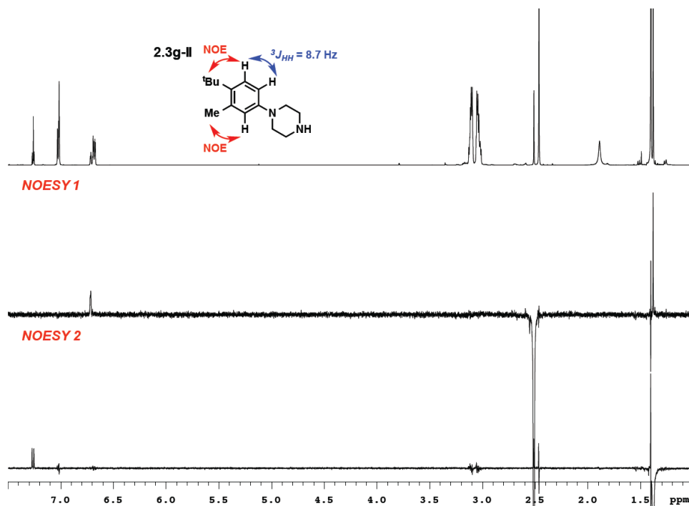
Figure E2.14. Structural assignment of 2.3g-II by 1-D NOESY NMR
