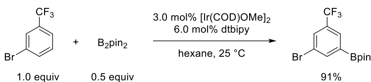
Figure I.4. Stoichiometric iridium-catalyzed borylation
