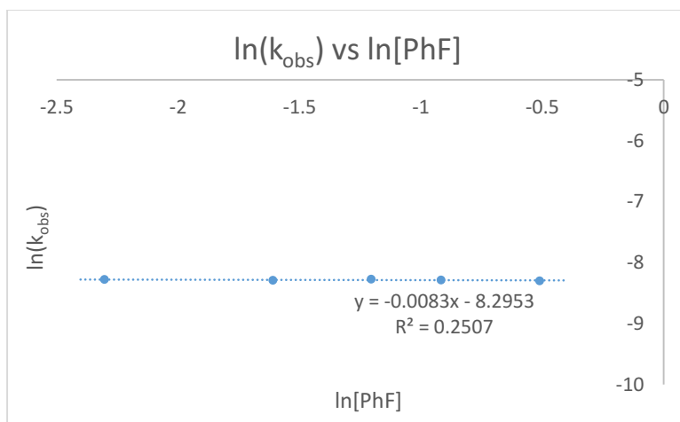
Figure E1.12. Determination of order in fluorobenzene
