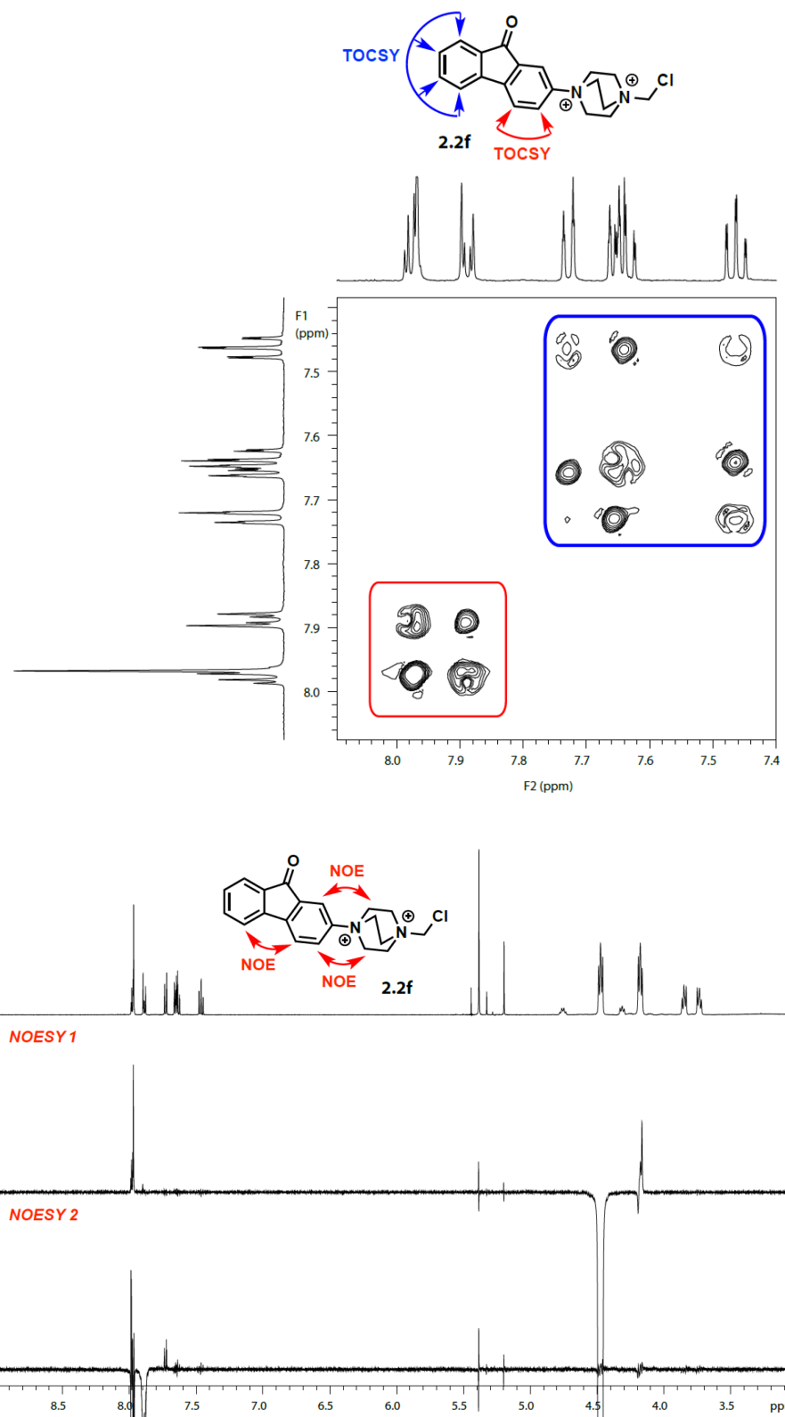
Figure E2.7. Structural assignment of 2.2f by TOCSY and 1-D NOESY NMR
