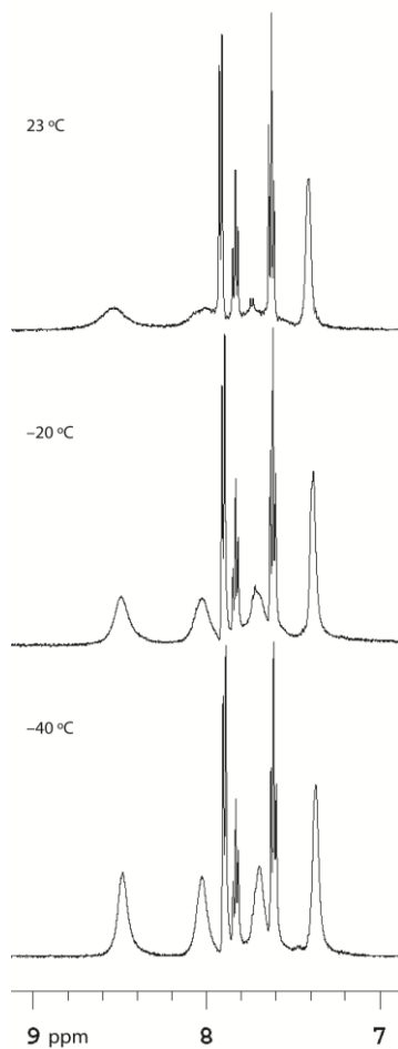
Figure E1.18. ^1\text{H} NMR peak broadness at 23 °C, -20 °C, and -40 °C ( \text{CD}_3\text{CN} , 23 °C)
