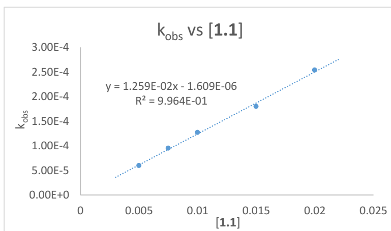
Figure E1.15. Determination of the second-order rate constant
