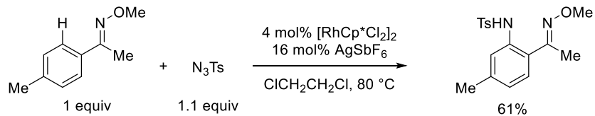
Figure I.2. Selected examples of chelation-assisted aromatic C–H functionalization 8-10
