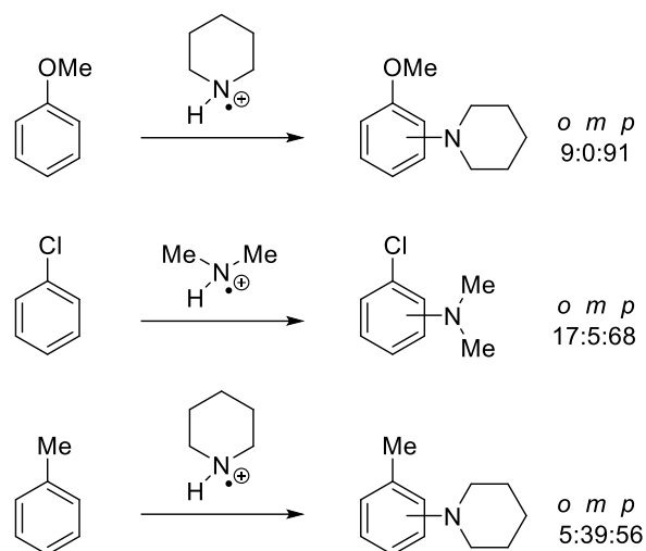
Figure I.7. Aromatic radical amination by cationic aminium radicals
