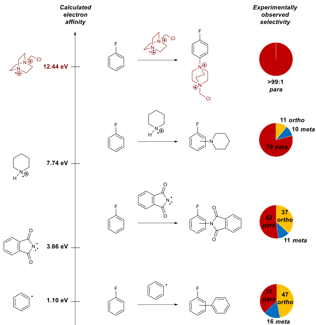
Figure 2.4. Selectivity for para substitution increases with increasing electron affinity of the radical. Electron affinities refer to gas phase adiabatic electron affinity calculated at the (U)B3LYP/6-311G(d) level of theory.
