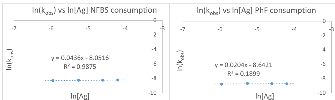
Figure E1.11. Determination of order in \text{Ag}(\text{bipy})_2\text{ClO}_4
