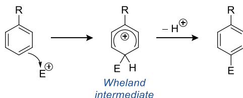
Scheme I.1. Mechanism of electrophilic aromatic substitution
