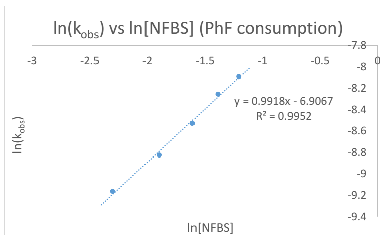
Figure E1.13. Determination of order in NFBS
