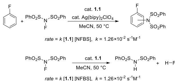
Figure 1.3. Kinetic studies of imidation and NFBS reduction catalyzed by 1.1
