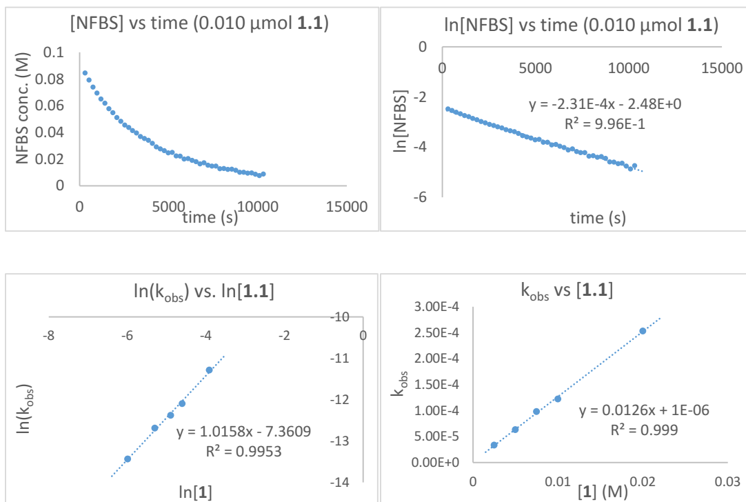
Figure E1.8. Kinetic data for determination of the rate law for NFBS reduction catalyzed by 1.1
