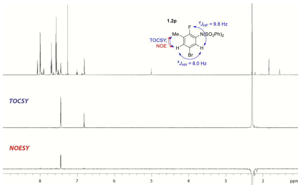
Figure E1.2. Structural assignment of 1.2p by 1-D TOCSY and NOESY NMR ( \text{CDCl}_3 , 23 °C)
