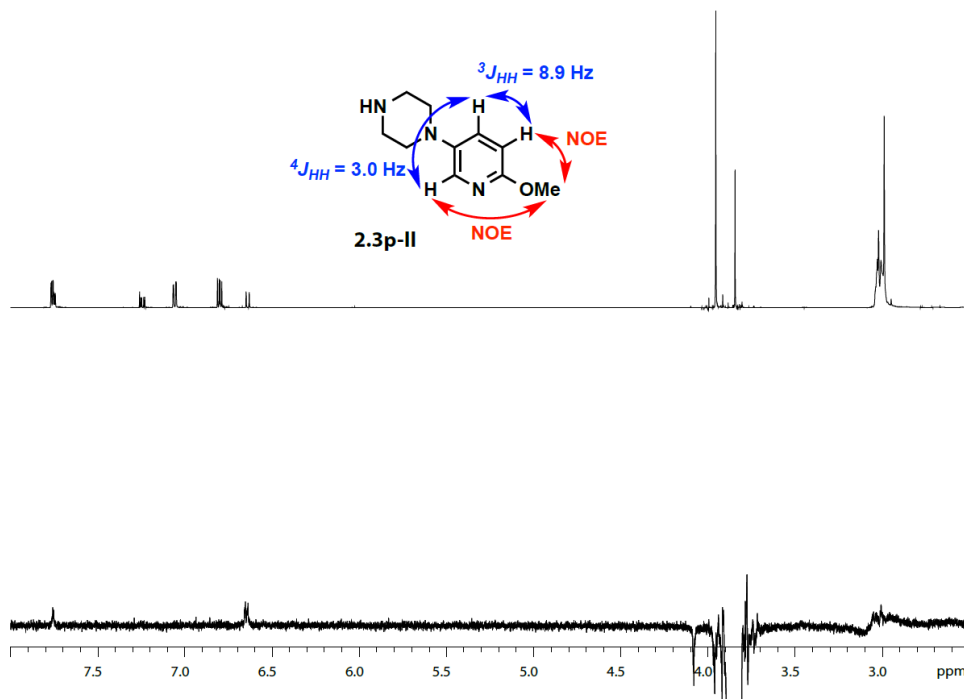
Figure E2.16. Structural assignment of 2.3p-II by 1-D NOESY NMR
