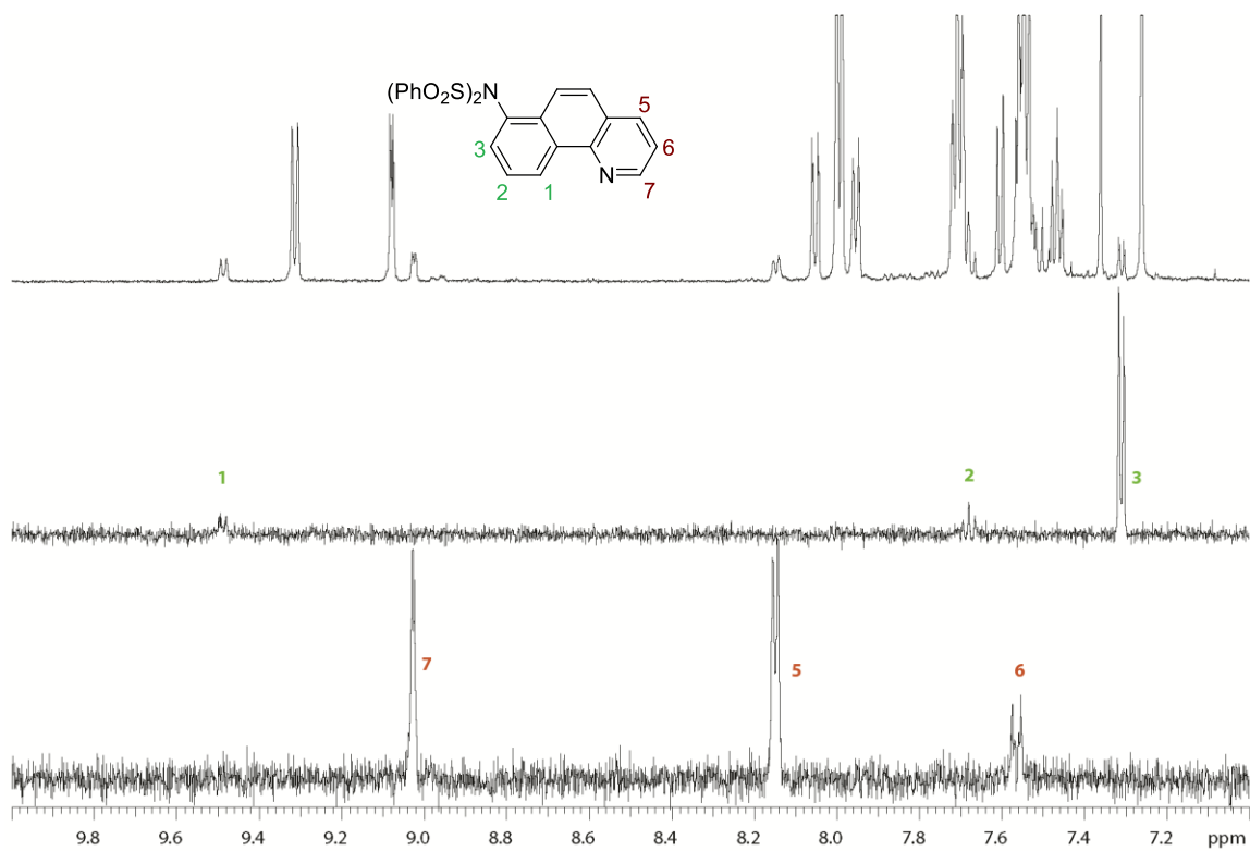
Figure E1.7. Structural assignment of 1.2q-III by 1-D TOCSY and NOESY NMR ( \text{CDCl}_3 , 23 °C)
