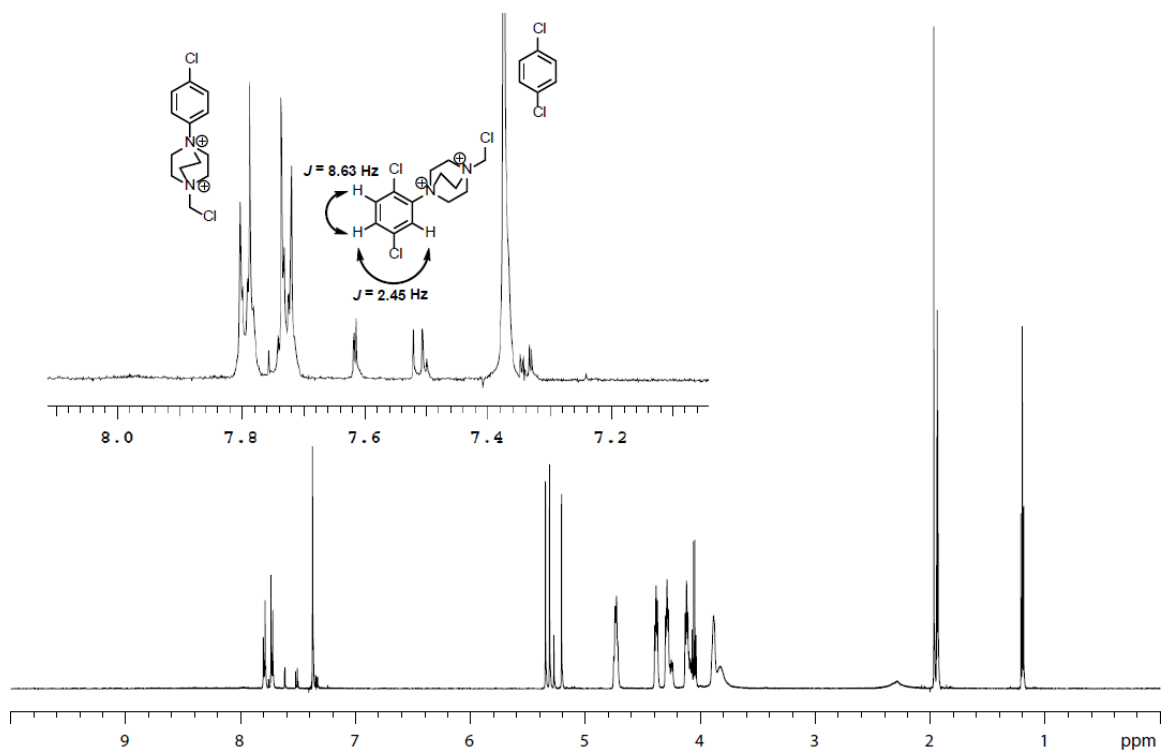
Figure E2.4. ^1\text{H} NMR of product mixture of TEDAylation of 1,4-dichlorobenzene ( \text{CD}_3\text{CN} , 23 ^\circ\text{C} )
