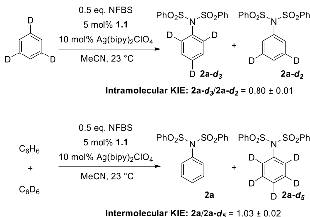
Figure 1.5. Intramolecular and Intermolecular Kinetic Isotope Effect
