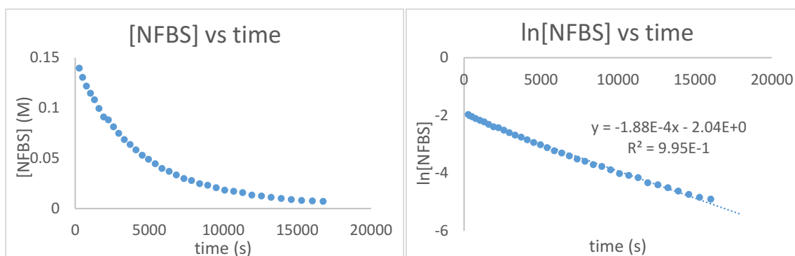
Figure E1.9. Time course of NFBS consumption in the imidation of fluorobenzene
