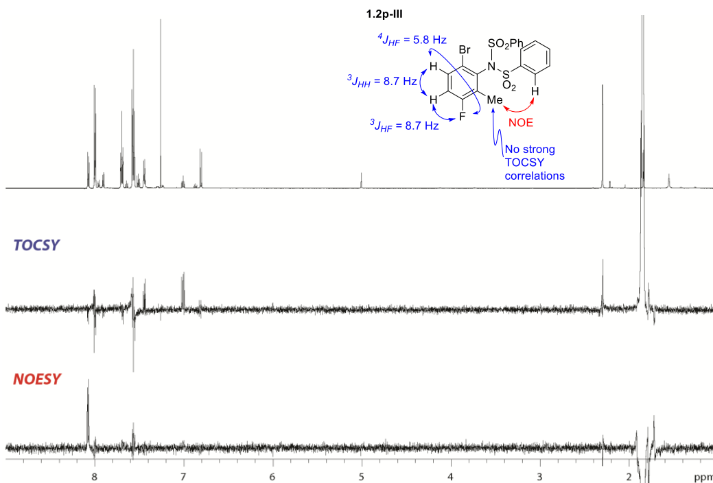
Figure E1.4. Structural assignment of 1.2p-III by 1-D TOCSY and NOESY NMR ( \text{CDCl}_3 , 23 °C)
