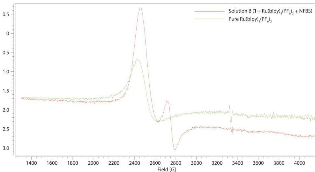
Figure E1.19. EPR spectra of Solution B and pure \text{Ru}(\text{bipy})_3(\text{PF}_6)_3
