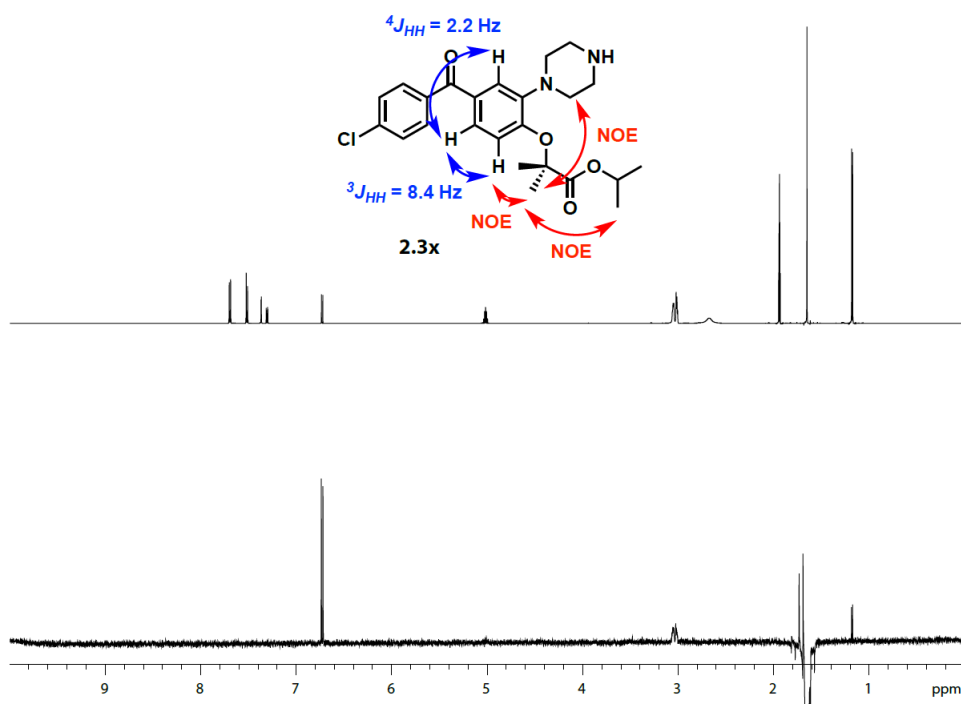
Figure E2.18. Structural assignment of 2.3x by 1-D NOESY NMR
