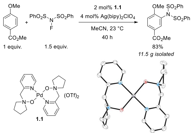
Figure 1.1. C–H imidation catalyzed by 1.1 and \text{Ag}(\text{bipy})_2\text{ClO}_4 , and x-ray structure of the cation of 1.1 (ellipsoids drawn at 50% probability)
