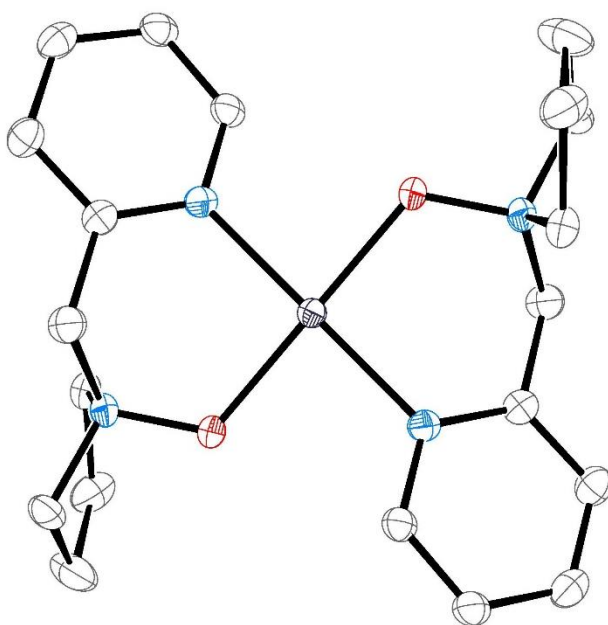
X-ray structure of 1.1 . Thermal ellipsoids are drawn at the 50% probability level; triflate anions and hydrogen atoms omitted for clarity
