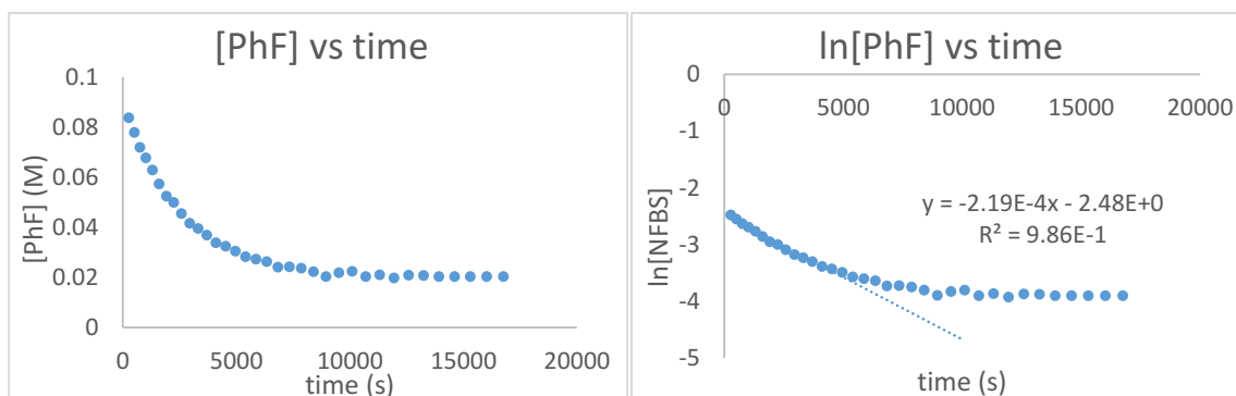
Figure E1.10. Time course of fluorobenzene consumption in the imidation of fluorobenzene.
