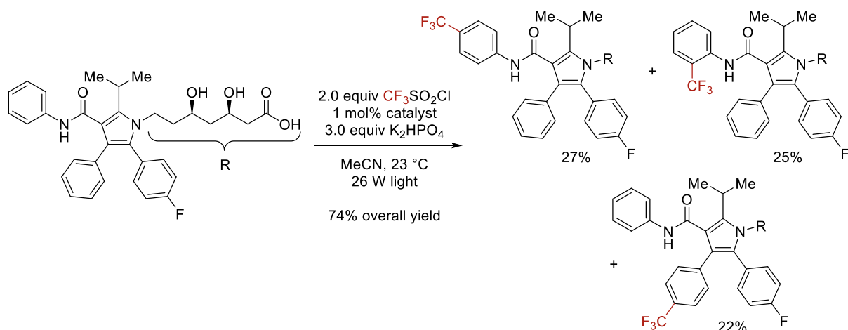
Figure I.9. Radical trifluoromethylation of Lipitor
