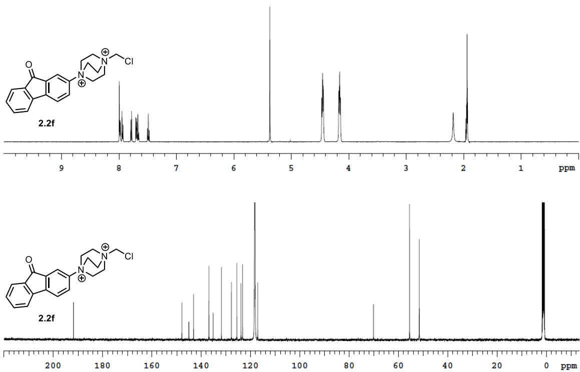
Figure E2.1. ^1\text{H} and ^{13}\text{C} NMR of pure Ar-TEDA 2.2f ( \text{CD}_3\text{CN} , 23 °C)
