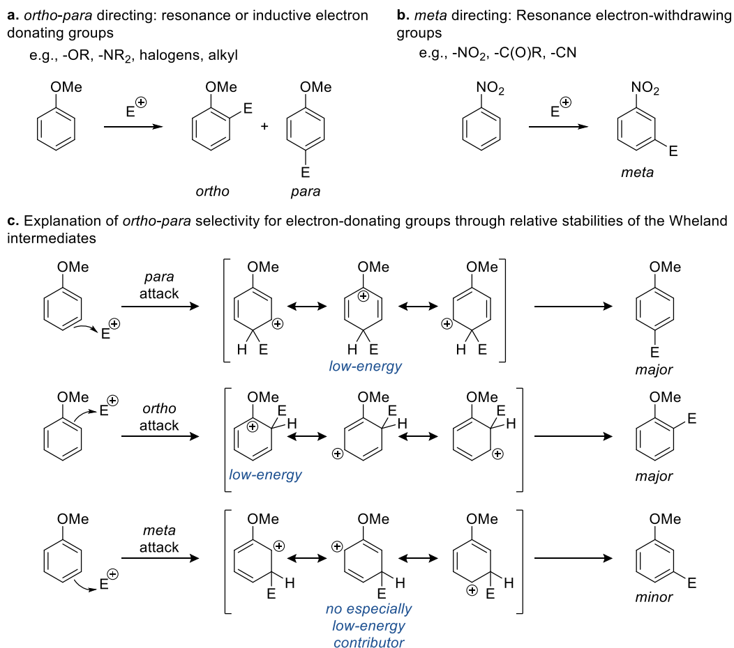
Figure I.1. Electrophilic aromatic substitution selectivity and rationalization through relative energetics of Wheland intermediates.
