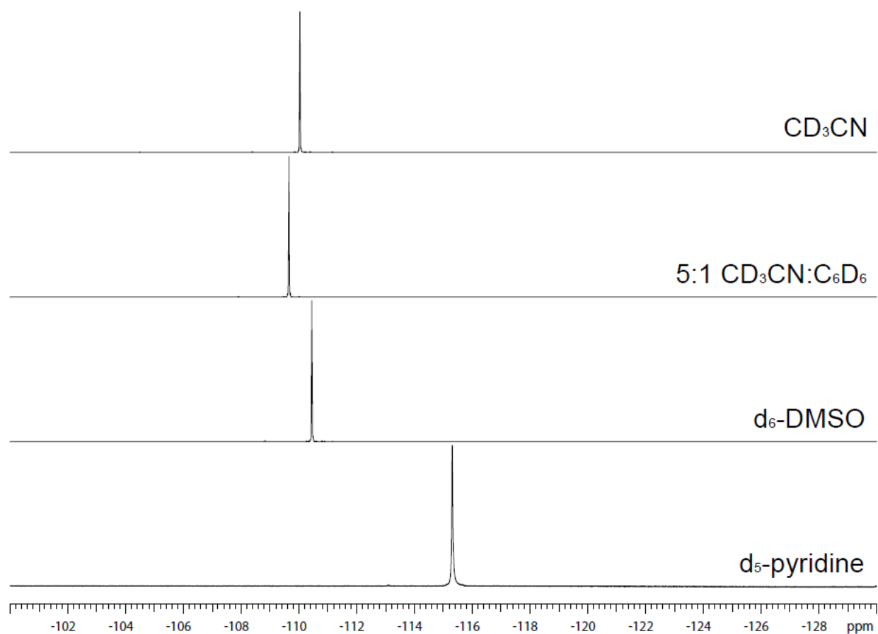
Figure E2.3. 19 F NMR evaluation of positional selectivity in different solvents (23 °C)
