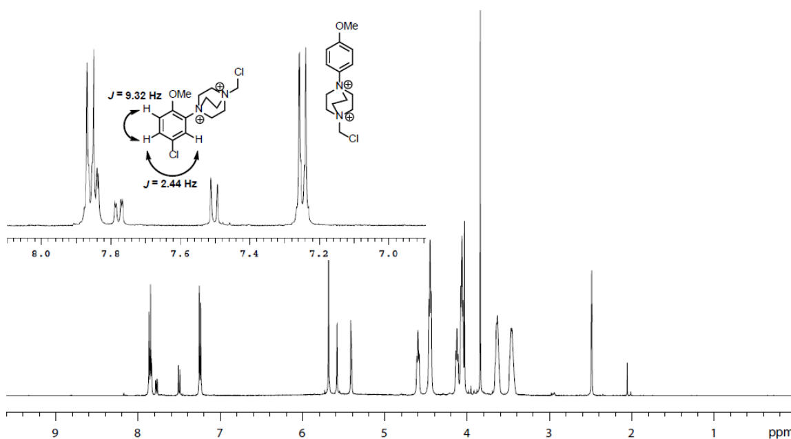
Figure E2.5. ^1\text{H} NMR spectrum of TEDAylation reaction mixture of 4-chloroanisole ( S )-1-(Chloromethyl)-4-(4-(2-(1,3-dioxoisindolin-2-yl)-3-methoxy-3-oxopropyl)phenyl)-1,4-diazabicyclo[2.2.2]octane-1,4-diium ( 2.2u )
