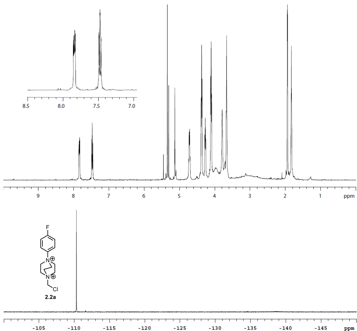
Figure E2.10. 1 H and 19 F NMR of 2.2a synthesized via copper catalysis (CD 3 CN, 23 °C)
