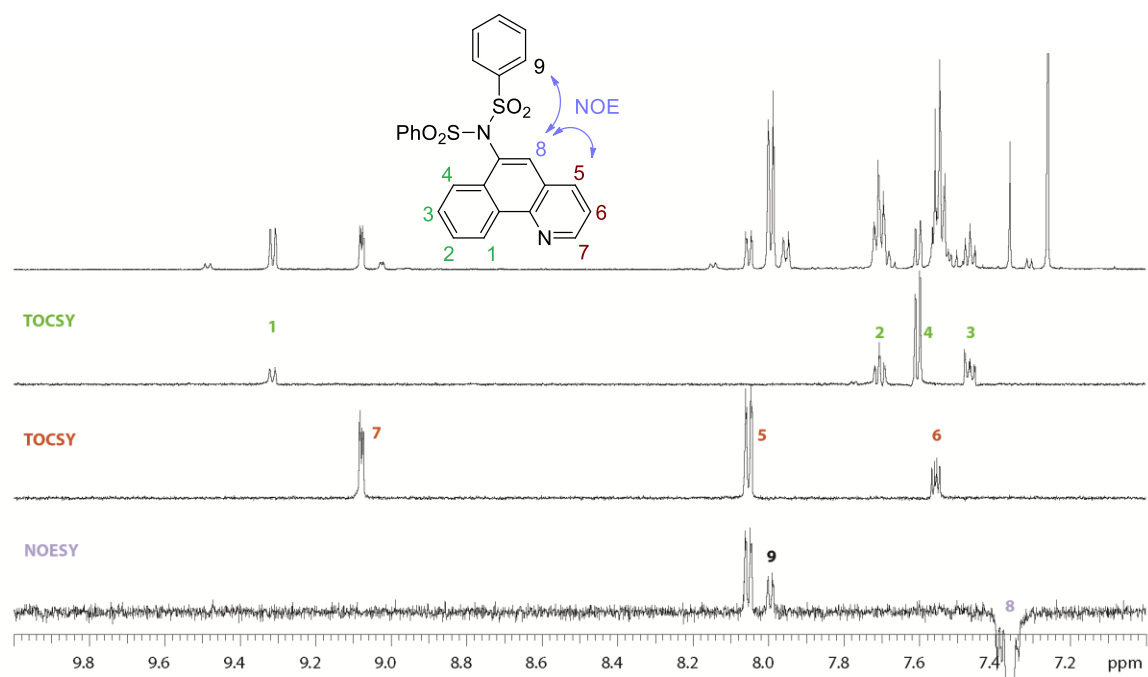
Figure E1.6. Structural assignment of 1.2q-II by 1-D TOCSY and NOESY NMR ( \text{CDCl}_3 , 23 °C)
