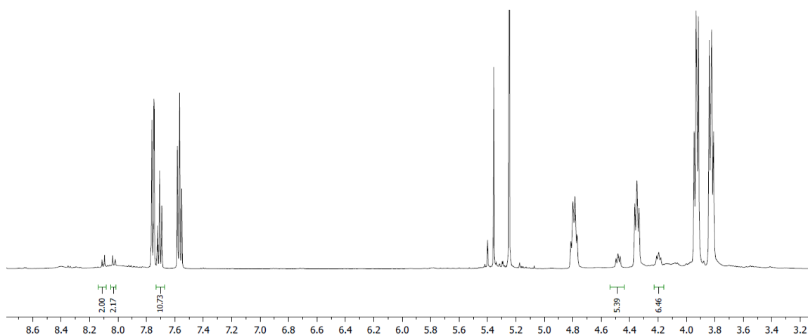
Figure E2.9. 1 H NMR of reaction mixture of TEDAylation of benzonitrile (CD 3 CN, 23 °C)
