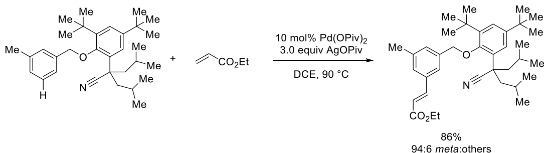
Figure I.3. Chelation-assisted meta -selective C–H functionalization
