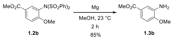
Scheme 1.1. Reduction of aryl sulfonamide products to anilines
