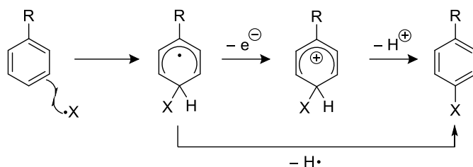
Scheme I.3. Mechanism of radical aromatic substitution
