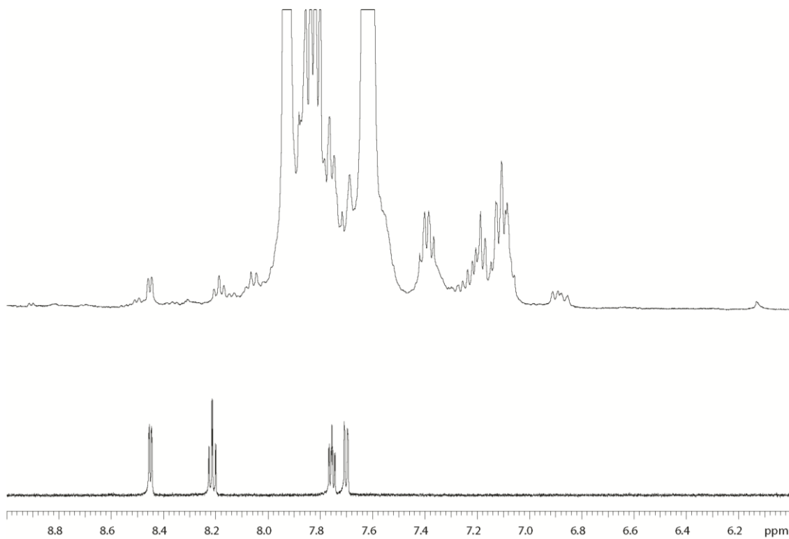
Figure E1.16. In-situ ^1\text{H} NMR of catalytic imidation (top), and pure 1.1 (bottom) ( \text{CD}_3\text{CN} , 50^\circ\text{C} )
