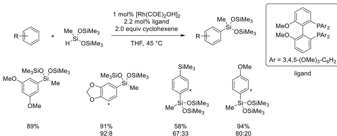
Figure I.5. Rhodium-catalyzed silylation with arene as limiting reagent
