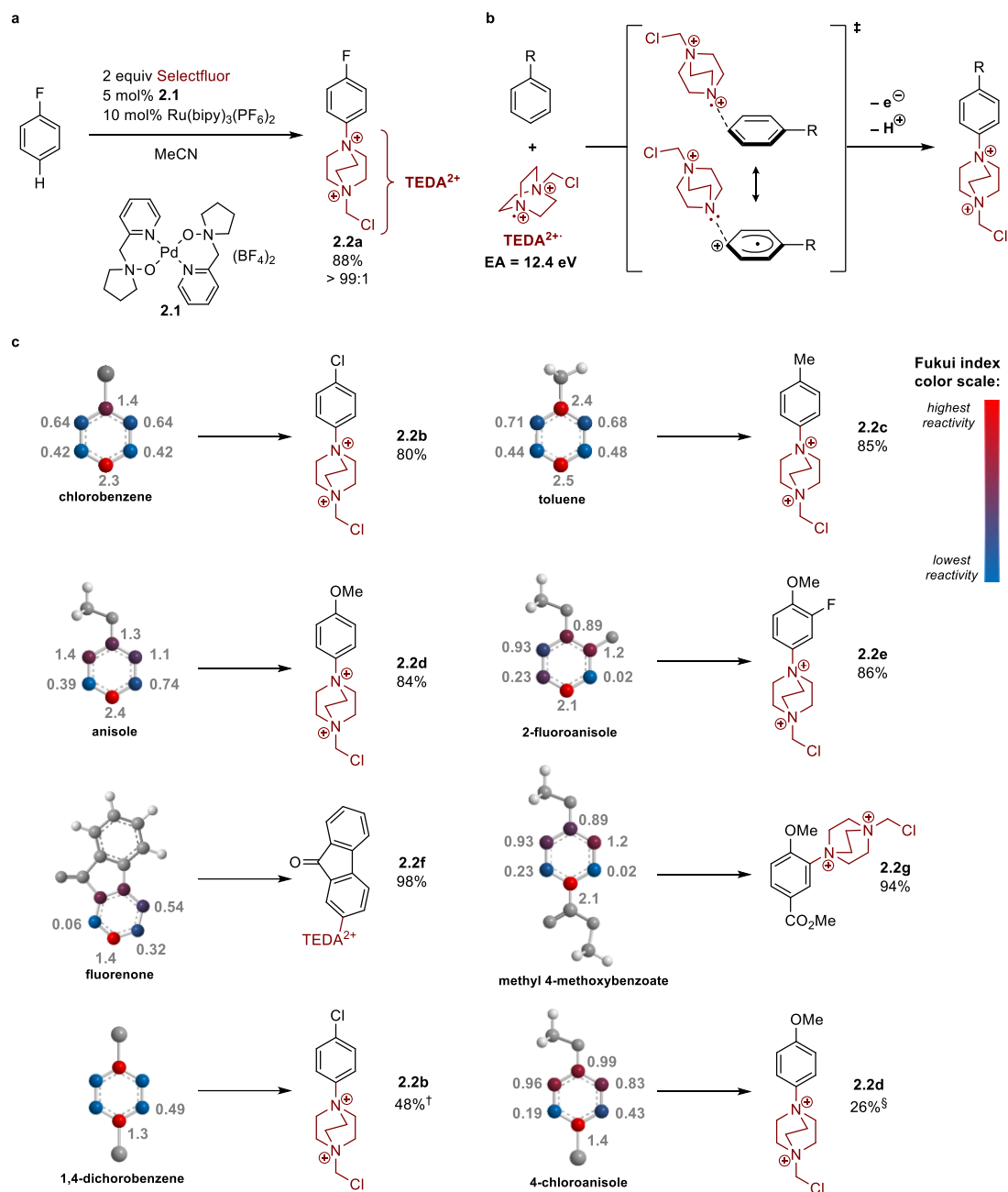
Figure 2.3. Charge transfer directed aromatic substitution. a , Conversion of fluorobenzene to the corresponding Ar–TEDA compound 2.2a . b , Positional selectivity of TEDA 2+ substitution is due to the stabilizing effect of arene-to-radical charge transfer in the transition state of addition. EA = Electron Affinity, refers to gas phase adiabatic electron affinity calculated by DFT. c , The position of substitution by TEDA 2+ is predictable by Fukui indices. Fukui indices depicted are multiplied by ten for simplicity of presentation. Note that Fukui indices are computed for one conformation of the molecule, so indices of positions that are symmetrically disposed about a substituent need not be equal. † Substitution in the 2-position was observed in 11% yield in addition to ipso substitution. § Substitution in the 2-position was observed in 10% yield in addition to ipso substitution.
