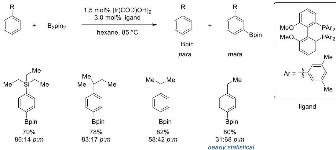
Figure I.6. Steric control of site selectivity in C–H borylation
