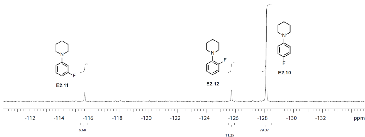
Figure E2.12. 19 F NMR analysis of product mixture of piperidine aminium radical substitution (CDCl 3 , 23 °C)
