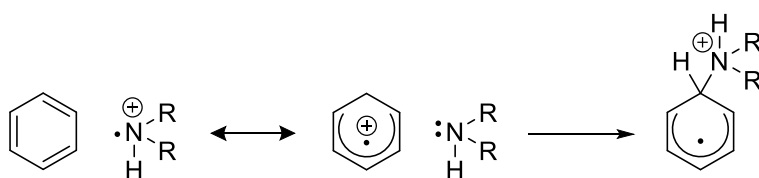
Figure I.8. Minisci's depiction of charge transfer contributions to radical addition. 19
