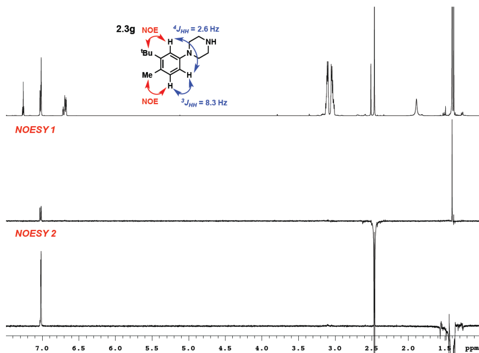
Figure E2.13. Structural assignment of 2.3g by 1-D NOESY NMR
