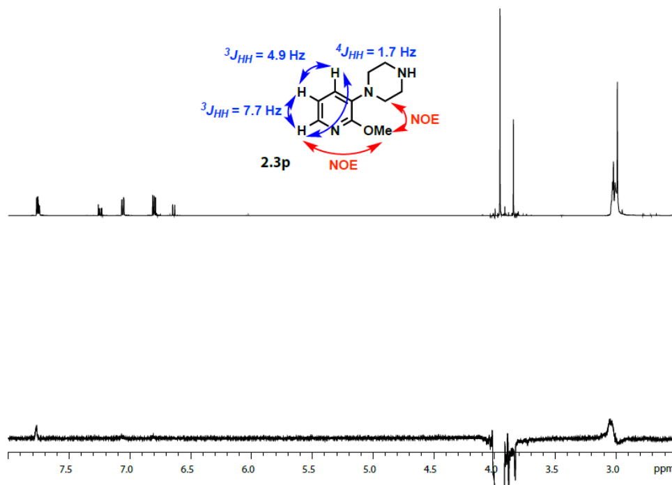
Figure E2.15. Structural assignment of 2.3p by 1-D NOESY NMR
