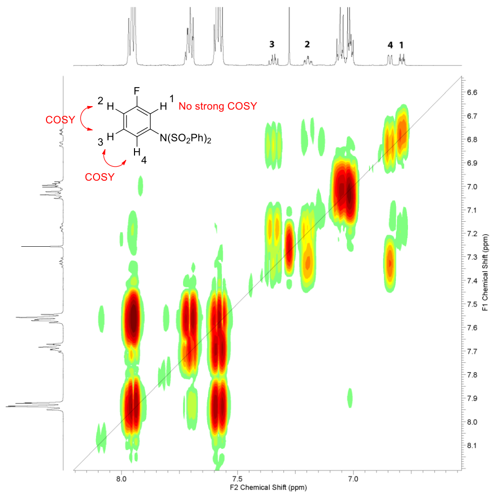
Figure E1.1. COSY for structural assignment of 1.2n-II ( \text{CDCl}_3 , 23 °C)
