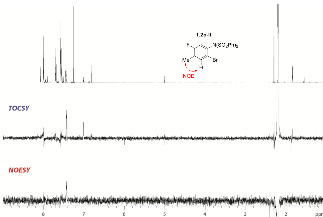
Figure E1.3. Structural assignment of 1.2p-II by 1-D TOCSY and NOESY NMR ( \text{CDCl}_3 , 23 °C)
