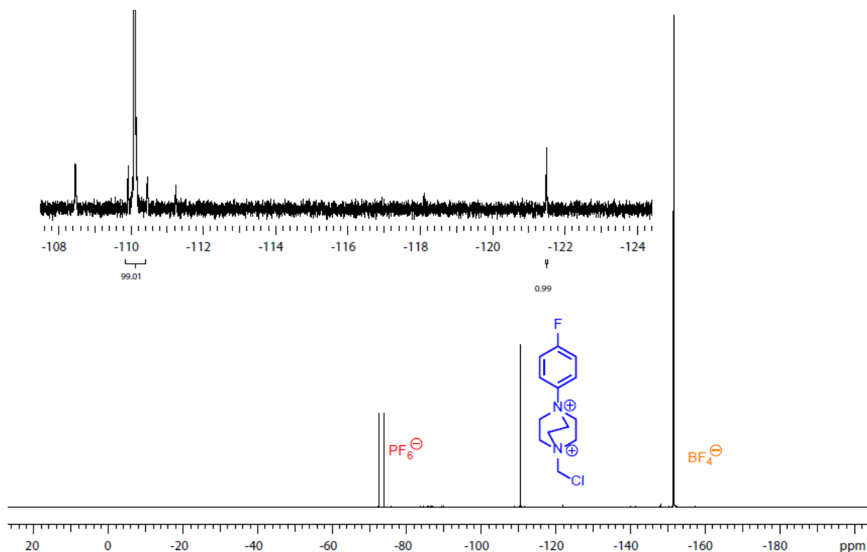
Figure 2.2. Determination of positional selectivity of TEDA addition to fluorobenzene by ^{19}\text{F} NMR. The next largest aryl fluoride peak after that of 2.2a has <1% intensity. See experimental section for full experimental details.
