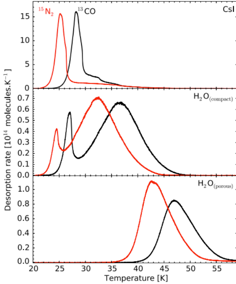
Figure 1.4: Desorption rate as a function of temperature in a TPD experiment, for CO and \text{N}_2 as pure ices (top panel), on a compact \text{H}_2\text{O} substrate (middle panel), and on porous \text{H}_2\text{O} substrate (bottom panel). The peaks in the desorption curves are at substantially higher temperatures for the water dominated ices. Reprinted with permission from Fayolle et al. (2016) .
