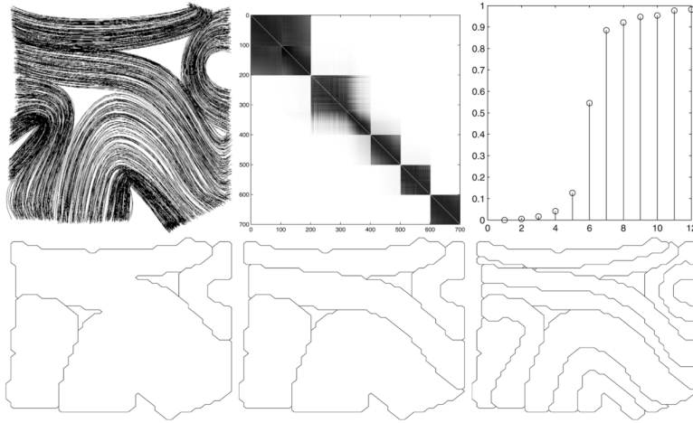
Fig. 2. Top left A set of synthetic fiber traces in 2-D. Top middle: The matrix W . Rows and columns sorted according to the second smallest eigenvector. The Gaussian kernel have been chosen so that five clusters present themselves naturally. Top right: The 15 smallest eigenvalues of (D - W)/D . Bottom: Segmentation obtained from recursive bipartitioning of the fiber traces. Maximum value of the N_{cut} set to 0.2, 2.5 and 4.5 respectively.
