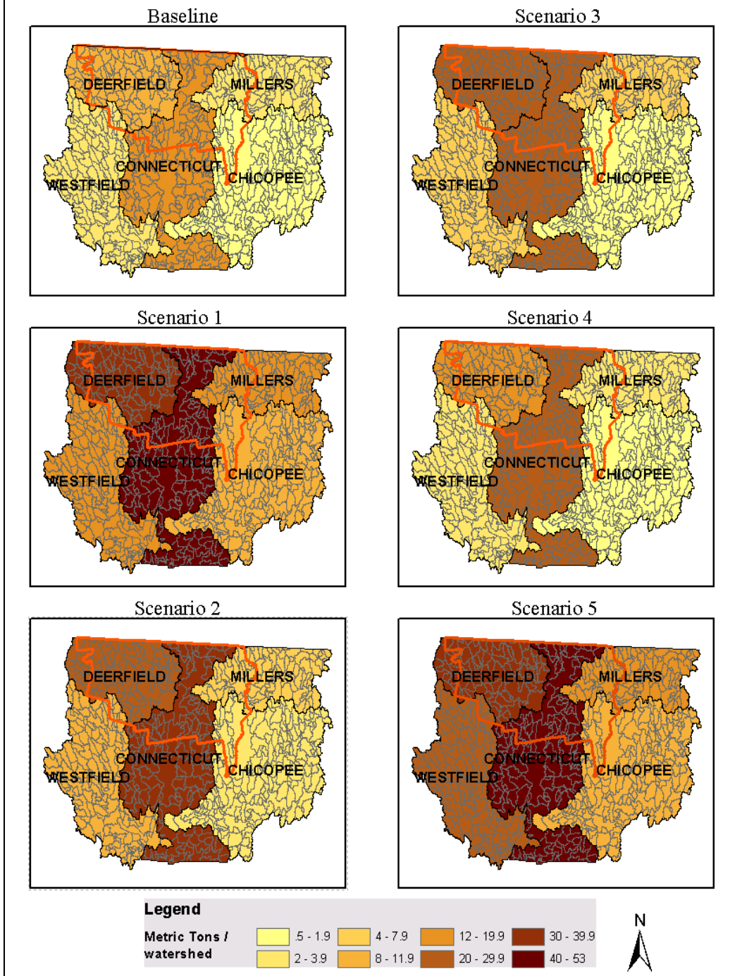
Figure 25. Relative changes in phosphorus export for each watershed. Note that each watershed drains into the Connecticut River Drainage Basin.
