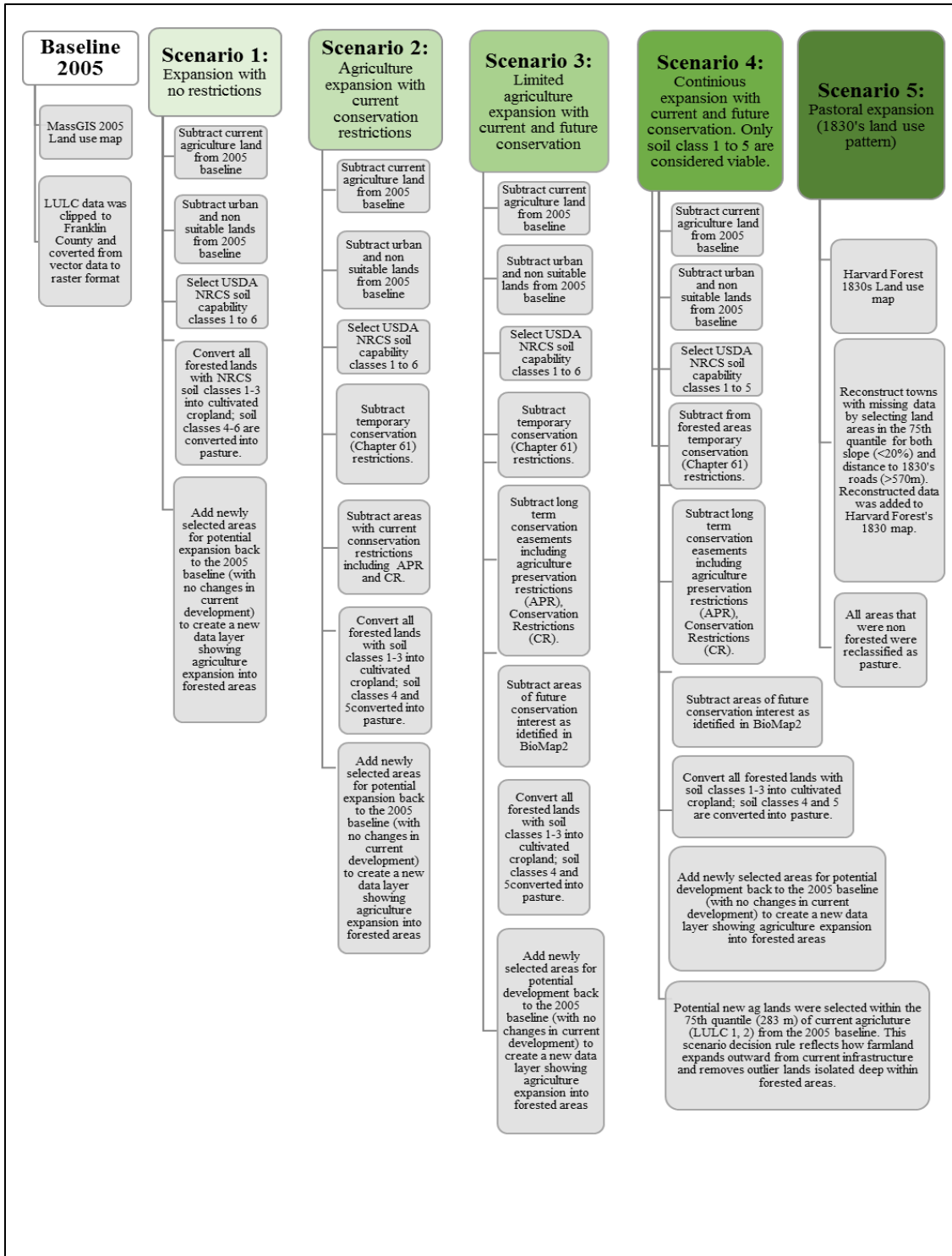
Figure 15. Flow chart showing the GIS procedures for each scenario.
