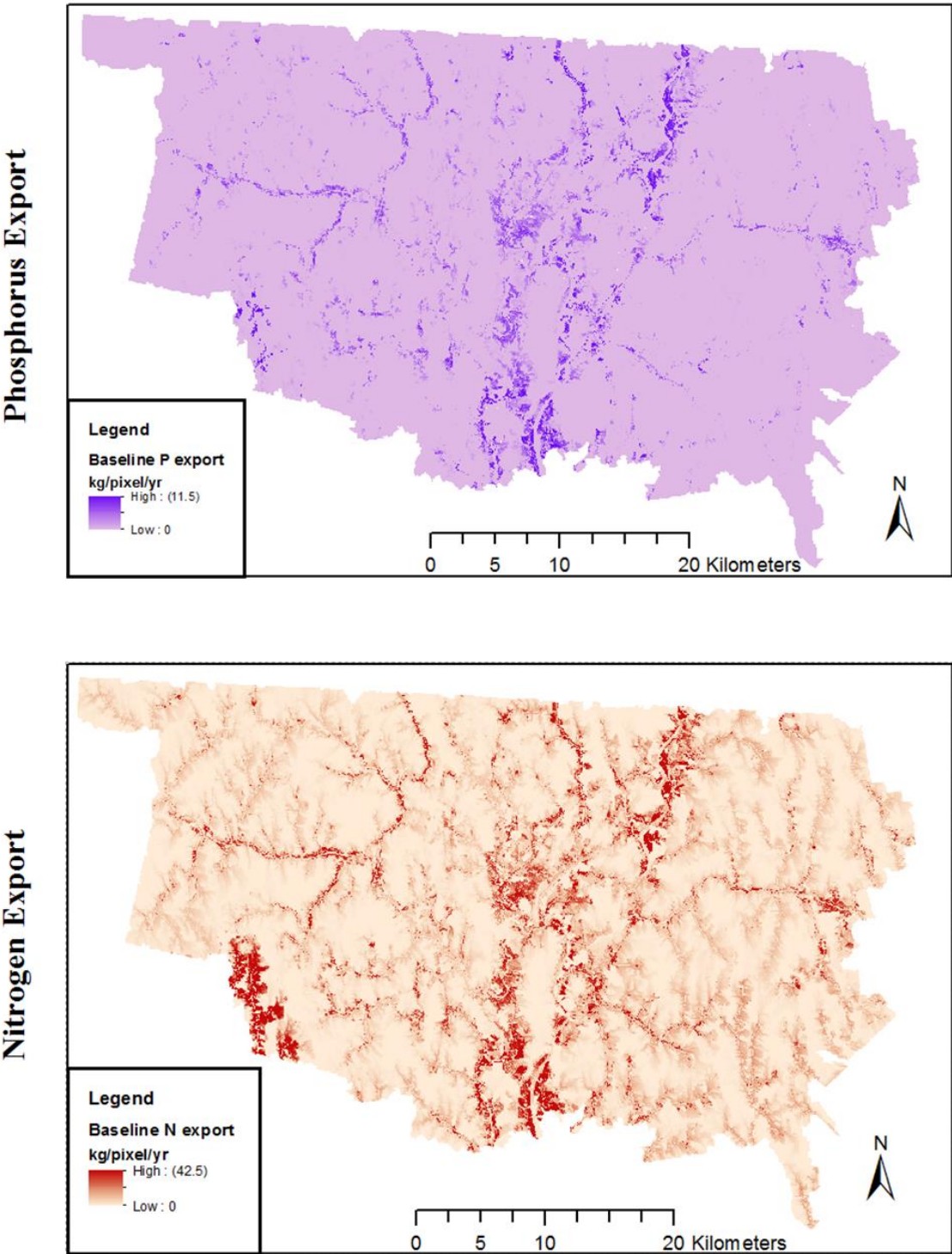
Figure 26. Map of baseline scenario nitrogen and phosphorus export. Note the geospatial distribution, in particular the heavy export in the south western portion of the county in the Westfield watershed.
