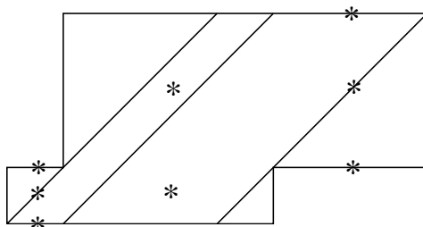
Figure 8. The spine of the foliation of slope 1 contains a pair of Weierstrass points.
