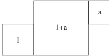
Figure 1. The polygon S(a) built from 3 squares.
