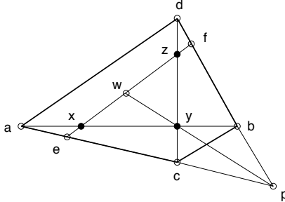
Figure 2. The triangle inequality.
