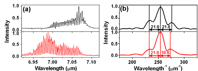
FIG. 1 (color online). (a) Spectra of a QCL with a 12\text{-}\mu\text{m} -wide active region. (b) Fourier transform of the spectra. The laser is driven by pulsed current I = 1.0 A (upper panel) and 0.75 A (lower panel) at a repetition rate of 80 kHz. The pulse duration is 125 ns.
