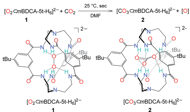
Fig. 1 The reaction scheme of peroxide cryptate 1 with \text{CO}_2 and a line drawing of [\text{O}_2\text{C}m\text{BDCA-5t-H}_6]^{2-} and [\text{CO}_3\text{C}m\text{BDCA-5t-H}_6]^{2-} .
