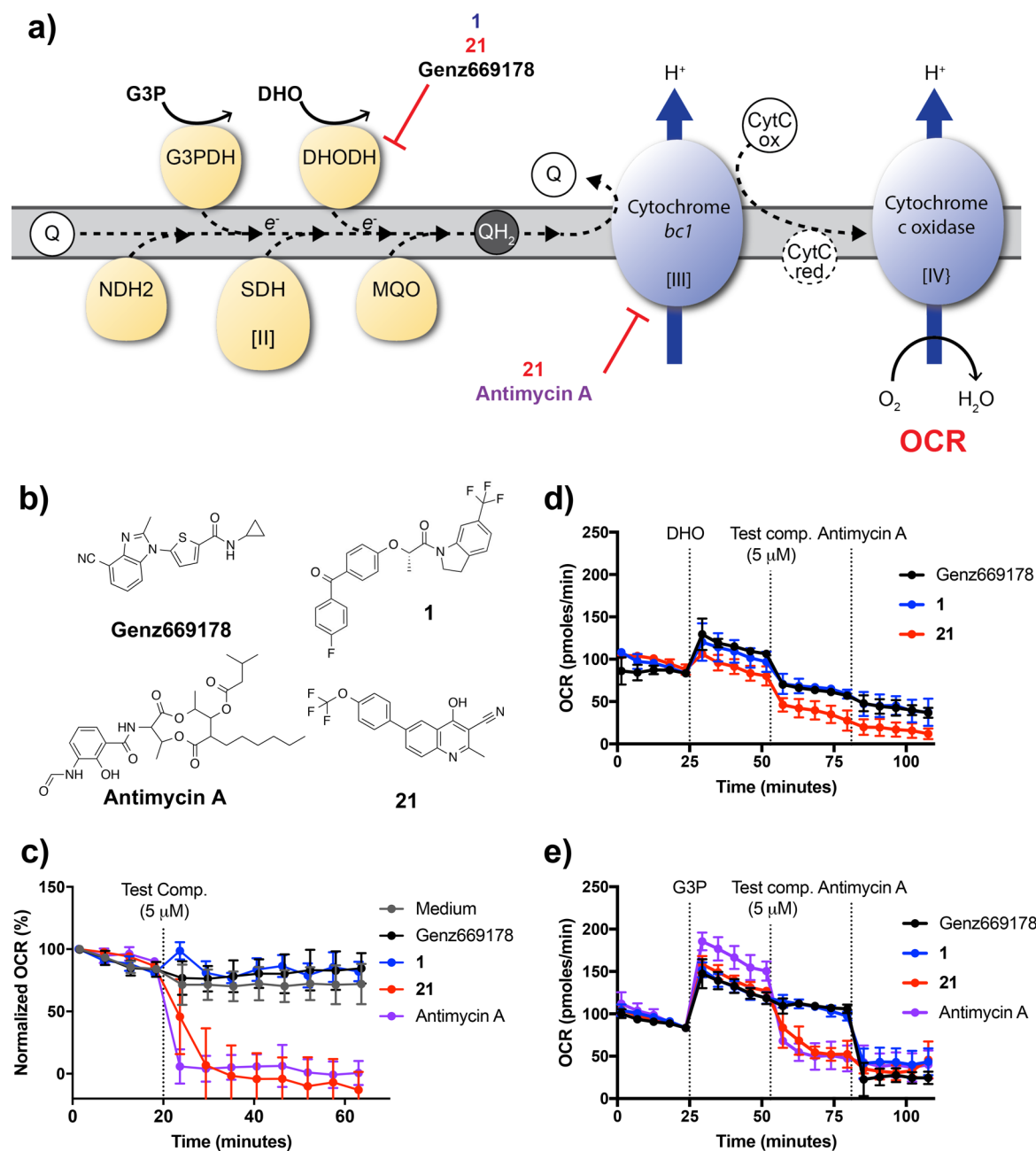
Figure 2. Extracellular flux analysis confirms the inhibitory activity of compound 21 against both PfCytbc 1 and PfDHODH . (a) A schematic representation of target identification using extracellular flux analysis. When G3P is provided as a fuel source, Cytbc 1 inhibitors such as antimycin A and compound 21 disrupt the electron flow of the ETC resulting in a reduction in the OCR. When DHO is the only fuel source provided, thus activating DHODH, electron flow and the OCR are reduced by DHODH inhibitors, such as Genz669178 and compounds 1 and 21 . (b) Structures of compounds tested in the extracellular flux assay. Genz669178 is a control DHODH inhibitor and antimycin A is a control Cytbc 1 inhibitor. (c) Antimycin A and compound 21 decreased OCR in RPMI media, indicating Cytbc 1 inhibition. Compound 1 and the DHODH inhibitor control Genz669178 do not have an effect on the OCR, similar to media-only controls. All data represent means \pm SD ( n = 3 ). (d) Compound 1 , compound 21 , and Genz669178 reduced the DHO-induced OCR, indicating their DHODH activity, while the Cytbc 1 inhibitor, antimycin A, did not. All data represent means \pm SD ( n = 3 ). (e) As observed in RPMI media conditions, only compound 21 and antimycin A reduced the OCR when G3P was the sole substrate. All data represent means \pm SD ( n = 3 ).
