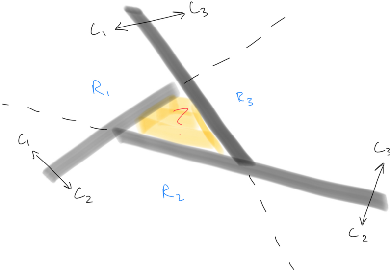
Figure 3.3: Ambiguities arise from one-versus-one method.
