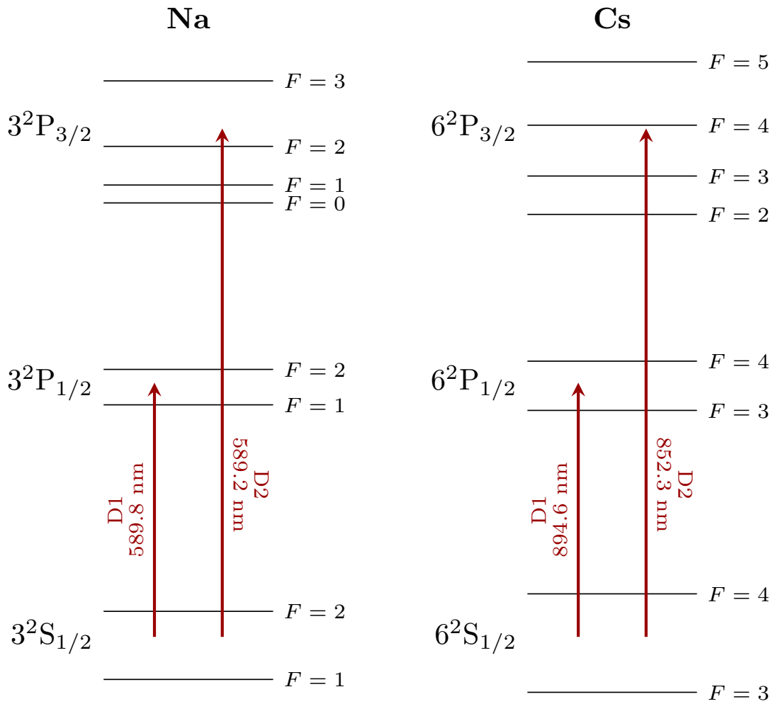
Figure 2.1: Energy diagrams for Na (left) and Cs (right) atoms including fine and hyperfine structures [89, 90]. Most of the cooling, state preparation and imaging steps use the D2 transition in our experiment with the exception of optical pumping (OP) on the sodium atom which uses both D1 and D2 lines (section 3.2.2).
