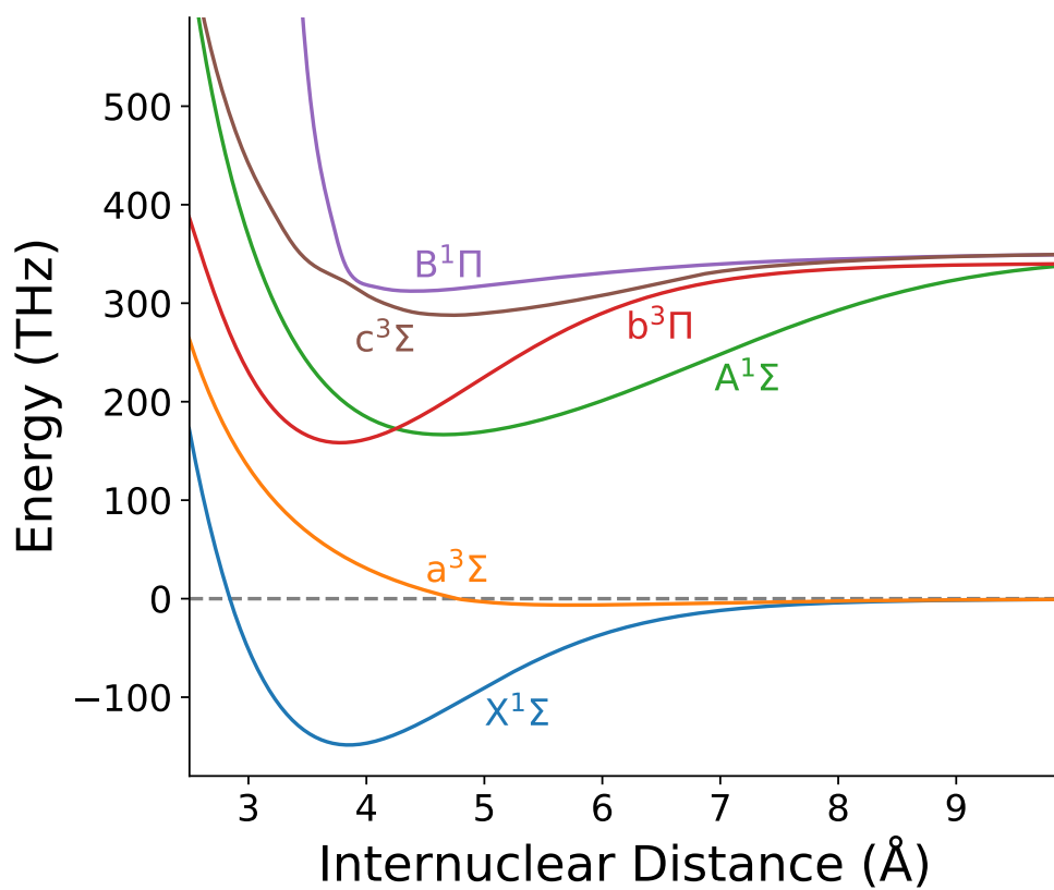
Figure 5.2: Potential energy surfaces of NaCs with Hund's case (a) labels [129, 134–136]. Due to spin-orbit coupling, the potentials are not independent of each other. The real energy eigenstates of the molecule may be a superposition of multiple electronic and spin states.
