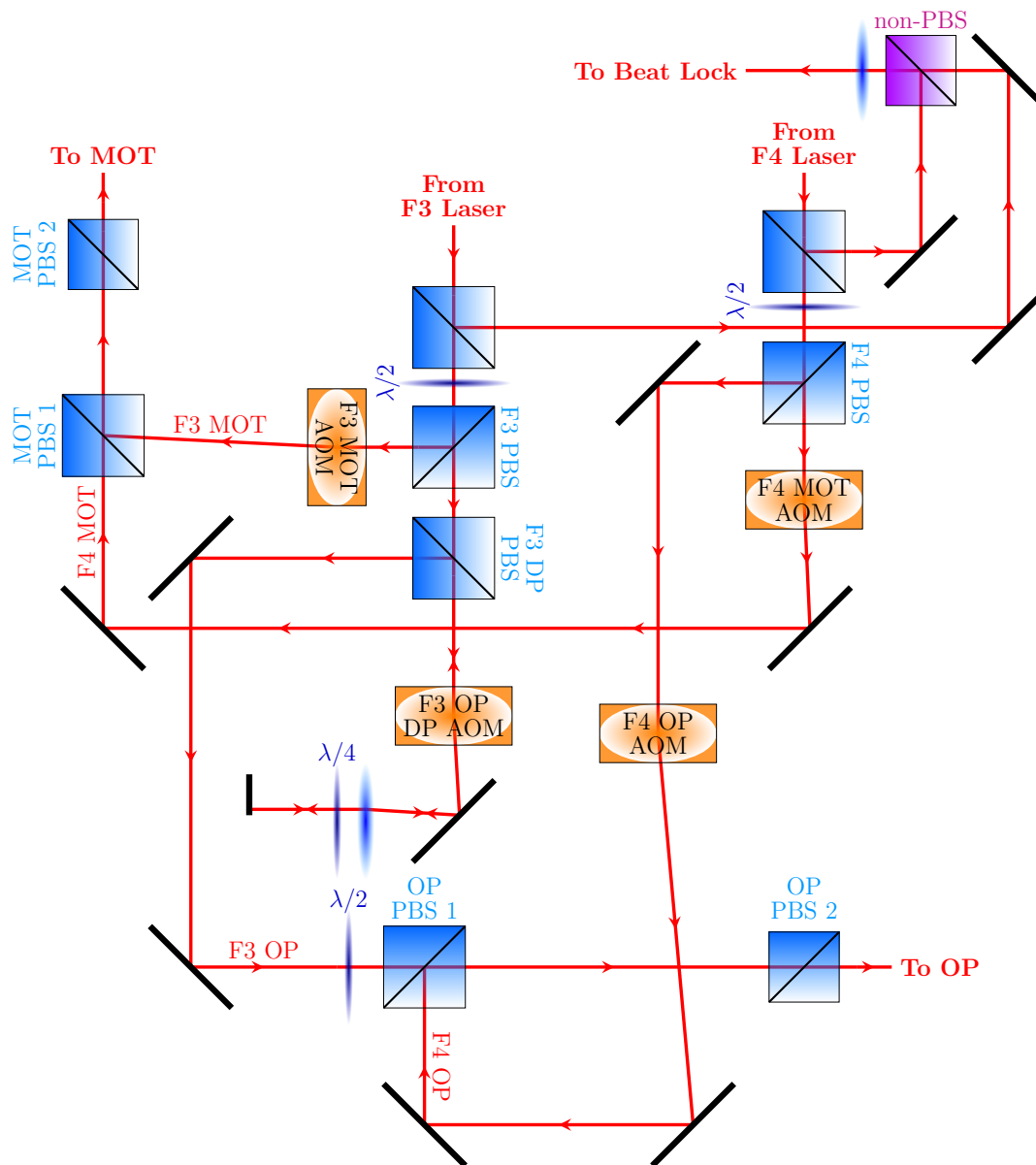
Figure 2.3: Beam path for generating the frequencies for Cs MOT and optical pumping (OP). (Beam path for fiber coupling and locking of the F 3 laser to the atomic transition is not shown.) The F 3 laser is locked using saturated absorption locking to the F 3 atomic transition. The F 4 laser is beat-locked to the F 3 laser, which also controls its frequency. The F 3 and F 4 light are combined on MOT PBS 1 and OP PBS 1 and their power ratio in the MOT and OP output are controlled by the rotating MOT PBS 2 and OP PBS 2 respectively. The frequency of the F 3 light in the MOT is fixed whereas the frequency of the F 3 light in the OP can be changed by the F 3 OP DP AOM.
