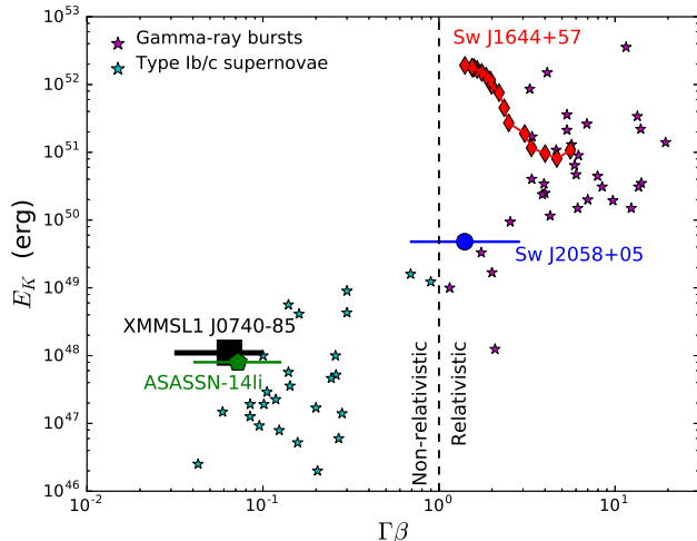
Figure 3. Kinetic energy ( E_K ) as a function of outflow velocity ( \Gamma\beta ) from radio observations of TDEs. We show the inferred values for XMMSL1 J0740–85 (black square; horizontal bar represents the range of velocity for a range of outflow geometries) as well as ASASSN-14li (green pentagon; Alexander et al. 2016) and the two \gamma -ray TDEs with radio emission: Sw J1644+57 (red diamonds; Zauderer et al. 2011 and Berger et al. 2012) and Sw J2058+05 (blue circle; Cenko et al. 2012). The data for Sw J1644+57 are from detailed modeling of the radio emission as a function of time, including a correction for jet collimation with an opening angle of about 0.1 rad (Zauderer et al. 2011; Berger et al. 2012). The data points and velocity ranges for Sw J2058+05 and ASASSN-14li are based on an identical analysis to the one carried out here (Alexander et al. 2016). Also shown for comparison are a sample of long-duration \gamma -ray bursts (LGRBs; magenta stars) and Type Ib/c core-collapse supernovae (Type Ib/c SNe; cyan stars) (Margutti et al. 2014).
