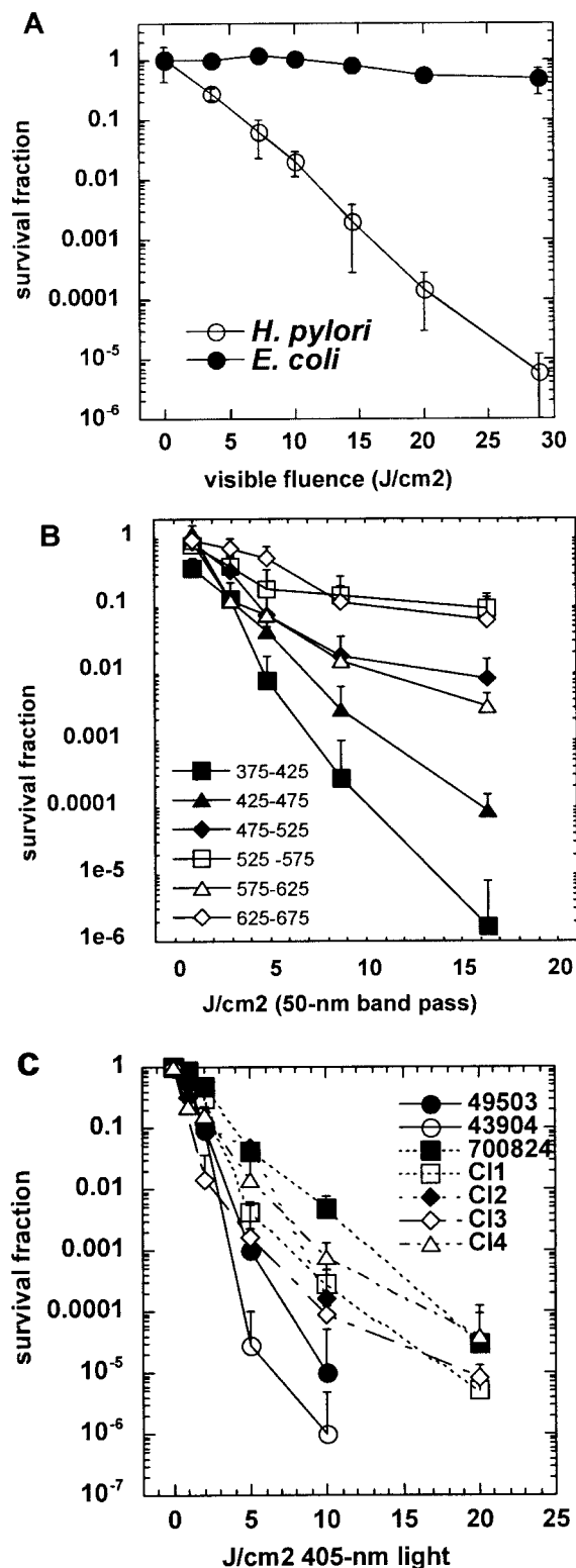
FIG. 1. A) Fluence-dependent killing of H. pylori ATCC 49503 after exposure to broad-band white light, >400 nm. E. coli is unharmed after similar illumination. Values are means of three independent experiments and bars are standard errors. B) Fluence-dependent killing of H. pylori ATCC 49503 after exposure to light produced by 50-nm band-pass filters. Values are means of three independent experiments and bars are standard errors. C) Comparison of photosensitivity of
