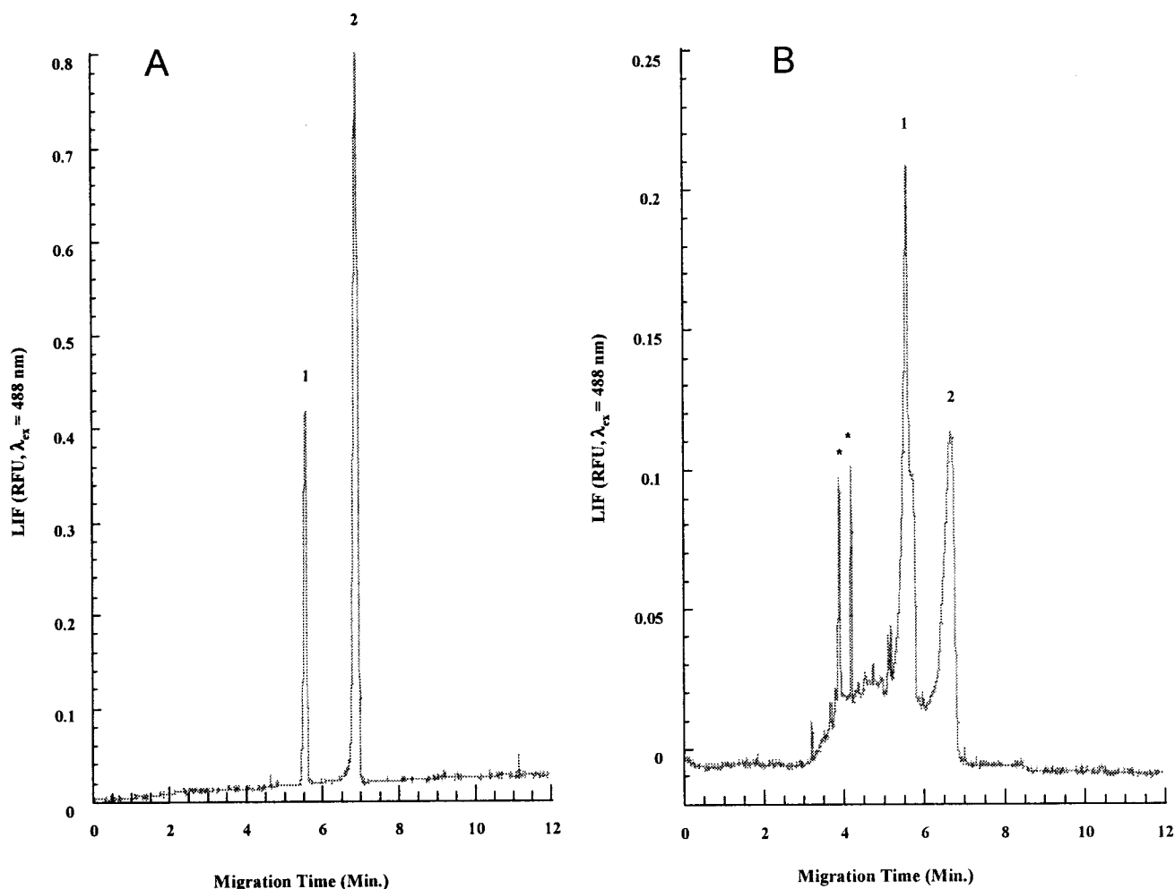
FIG. 3. A) Capillary electrophoresis of standard mixture of CP (peak 1) and PPIX (peak 2). B) Capillary electrophoresis of extract from culture supernatant of 4-day-old H. pylori ATCC 49503. Peaks marked * may be artifacts or very low concentrations of porphyrins with more than four carboxyl groups.
