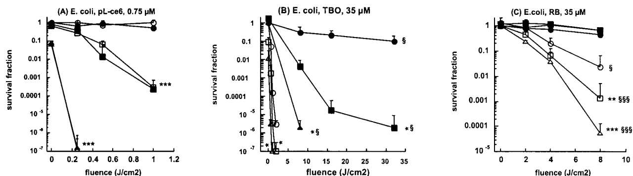
FIG. 3. Photoinactivation of E. coli . Cells were incubated with the specified concentration of PS for 20 min followed by illumination with the appropriate wavelength of light (see text). ● and ○, 10^9 cells/ml; ■ and □, 10^8 cells/ml; ▲ and △, 10^7 cells/ml; ●, ■, and ▲, PS washed from cells before illumination; ○, □, and △, PS left in cell suspension during illumination. The values shown are means of three independent experiments, and bars are the standard error of the mean. ***, P < 0.001 ; **, P < 0.01 ; *, P < 0.05 , compared with next highest cell concentration. $$$, P < 0.001 ; and §, P < 0.05 , between no wash and corresponding wash.
