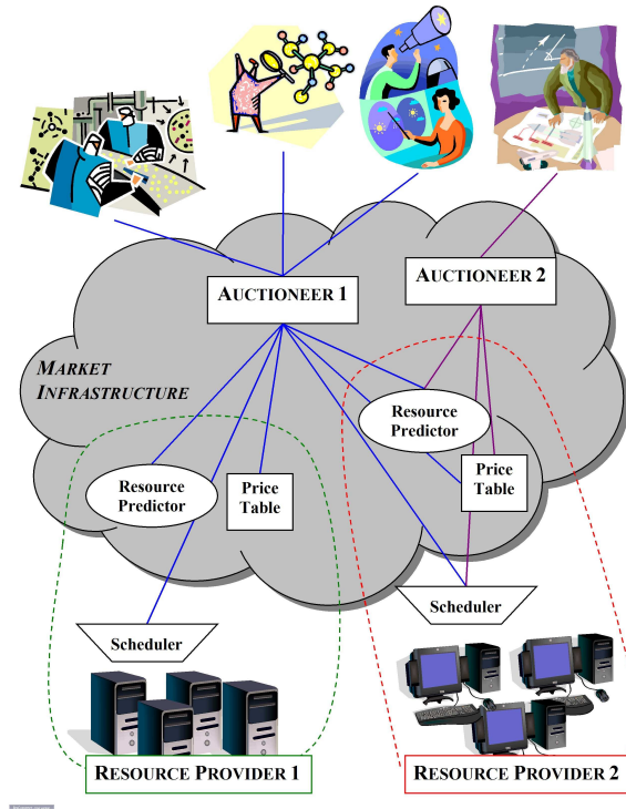
Figure 1: Actors
