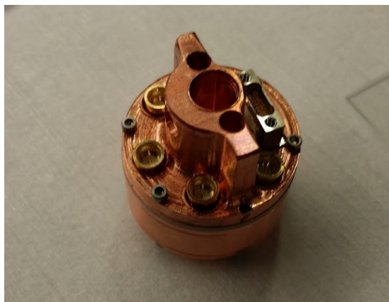
Figure A.4: Sample package mounted to the custom adapter made for the Oxford cryostat. Adapter has two machined holes to house a heater and thermometer. Entire package is then affixed to the end of a long SS thin-walled tube and lowered into the Oxford VTI.
