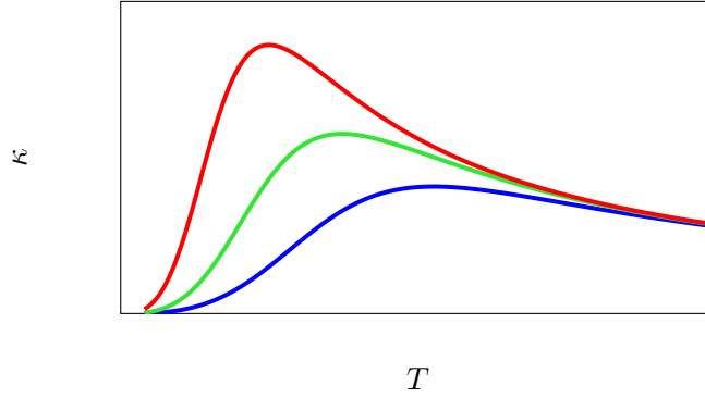
Figure 7.10: A sketch of \kappa(T) , accounting for coupling to acoustic phonons, for samples of graphene with three different amounts of disorder (measured by u ). We take a = 3, b = 1 in this plot.
