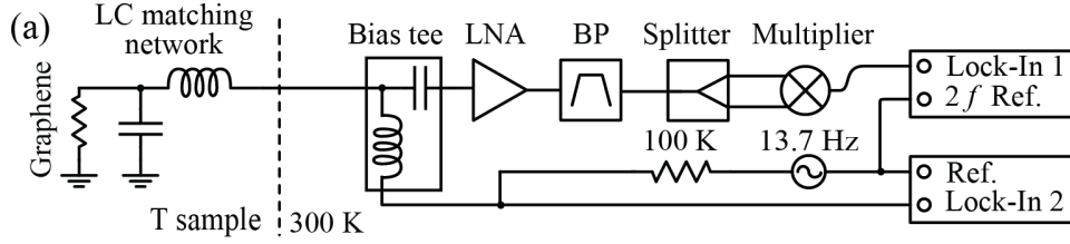
Figure 4.4: Simplified schematic of thermal conductance measurement setup. A low frequency Joule heating current is pass through the sample using a lock-in amplifier and the corresponding temperature is measured using Johnson noise thermometry. A bias tee is used to combine the DC and RF signals. The noise signal is measured as the second harmonic of the heating current as \Delta T \sim I^2
