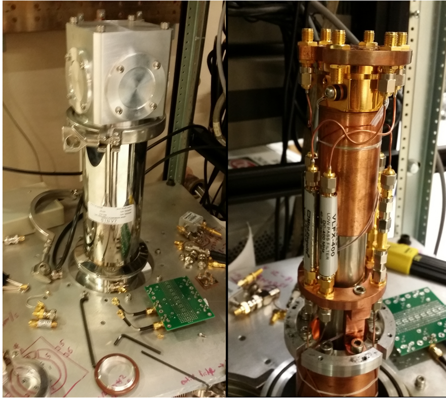
Figure A.3: Janis SHI-4 cryocooler used in parts of this dissertation. (Left) image of the closed system sealed and under vacuum. Optical windows are available but are blocked for these experiments. (Right) image of the opened system exposing the RF semi-rigid coax cables. The sample package is mounted onto the top plate which is cooled via a closed cycle ^4\text{He} system and the temperature is set using a heater, thermometer, and Lakeshore PID controller. Low-pass filters are placed at the mid temperature plate to reflect room temperature noise.
