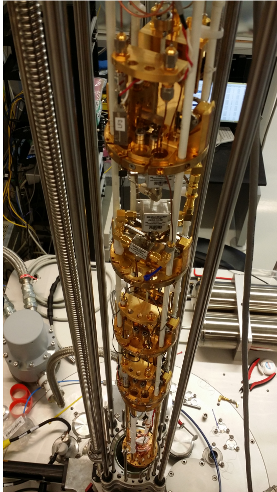
Figure A.13: An image of a microwave noise measurement circuit installed on the Leiden probe. A low noise amplifier is mounted to the 4\text{ K} plate and a bias-tee along with two directional couplers are attached. This setup allows RF reflection and gain measurements of the sample and amplifier, respectively, as well as DC transport and RF noise measurements.
