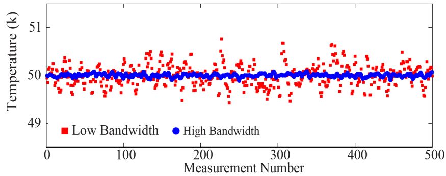
Figure 2.7: 500 repeated Johnson noise measurements of a 50\ \Omega resistor at 50\ K using two different measurement bandwidths. The high bandwidth data has smaller statistical fluctuations than the low bandwidth data.
