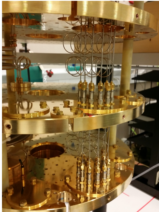
Figure A.11: Image of the microwave lines inside in the body of the Leiden cryostat. Shown here are the 14 excitation lines connecting the still plate to the mixing chamber plate attenuated at every stage. Not shown are the 2 superconducting measurement lines installed alongside these without attenuators.
