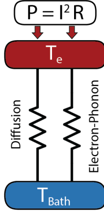
Figure 4.1: Simplified thermal diagram of the electronic cooling pathways in graphene relevant for the experimental conditions presented here. A current induces a heating power into the electronic system which conducts to the bath via two parallel pathways: diffusion and coupling to phonons.
