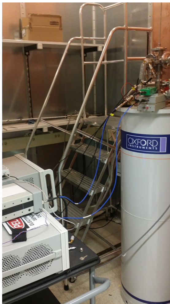
Figure A.6: Image of the Oxford cryostat with VTI and RF probe during a measurement. All electronics are kept at room temperature. The entire fridge is housed inside a shielded metal room.
