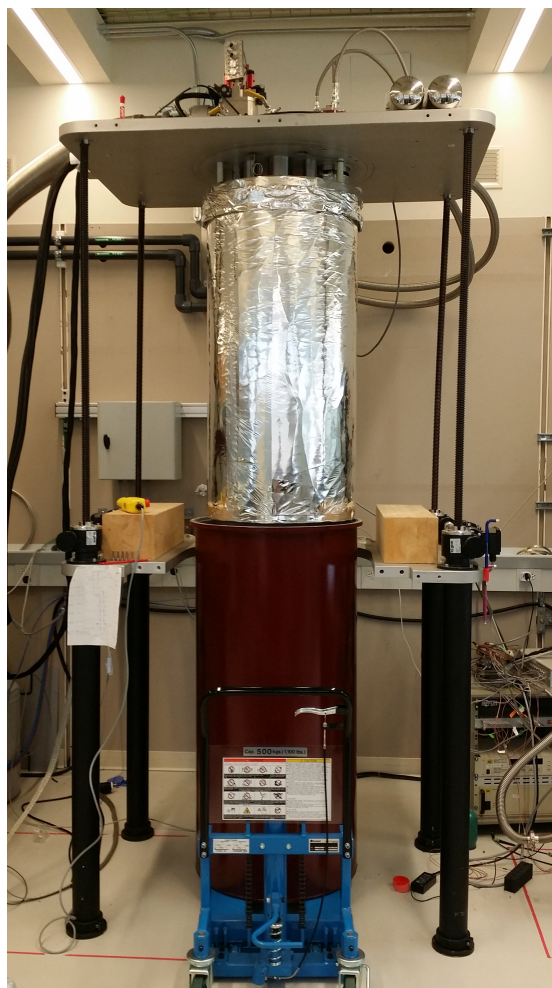
Figure A.8: Image of the Leiden cryostat being disassembled. The four electrically controlled legs are extended, lifting the entire system for easy maintenance.
