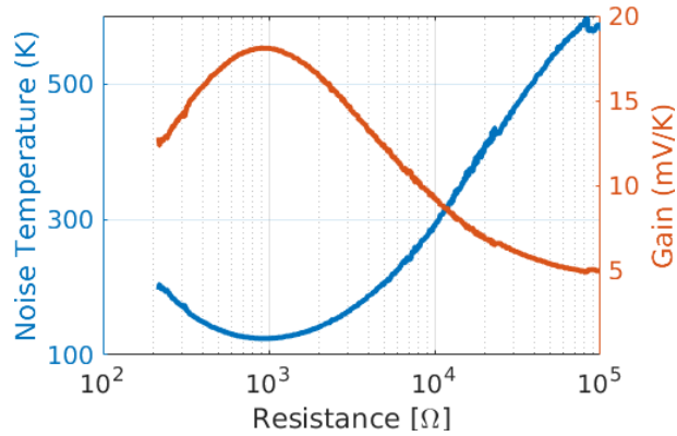
Figure 2.24: Generalize gain and effective noise temperature extracted from data shown in Fig. 2.23. The circuit is designed to optimally match an input resistance of \sim 1\text{ k}\Omega . As expected from Eqn. 2.26 and 2.27, the gain is maximized and the noise temperature is minimized when the device is effectively coupled — i.e. \Gamma is minimized. This two-stage LC tank circuit shows effective coupling over 3 orders of magnitude of input resistance.
