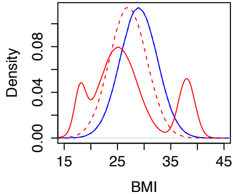
Trimodal
