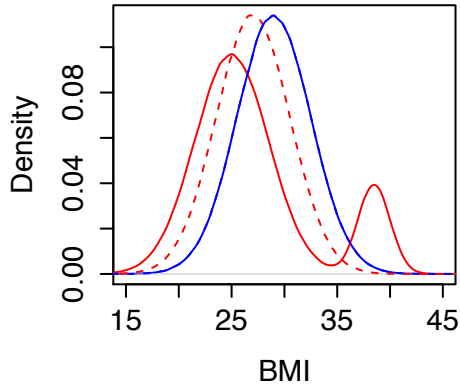
Bimodal
