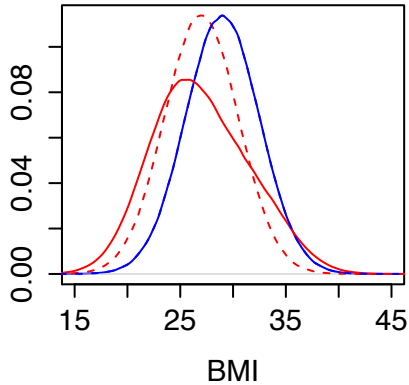
Right Tail
