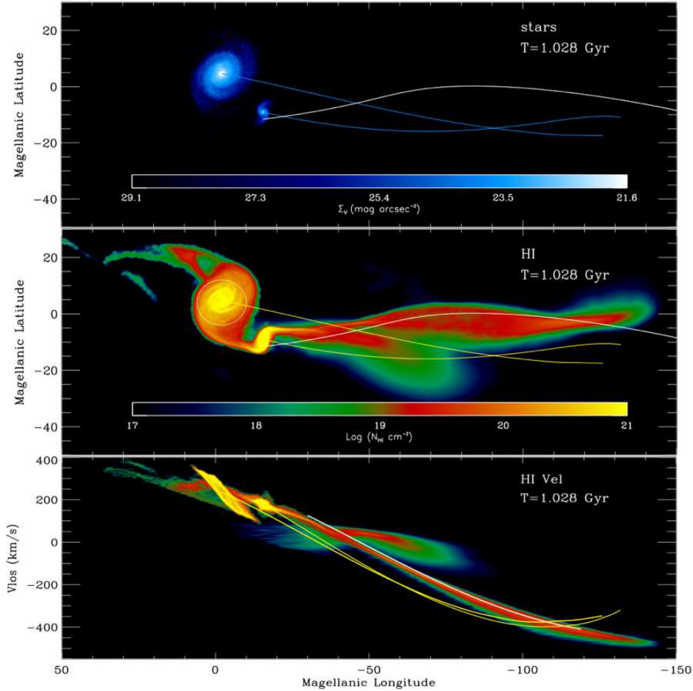
Fig. 2.— The stellar surface brightness, HI gas column densities and line-of-sight velocities of the simulated Magellanic system. Top panel: The resulting stellar distribution is projected in Magellanic coordinates (N08), a variation of the Galactic coordinate system where the Stream is straight. The distribution is color-coded in terms of Vband surface brightness. The past orbit of the L/SMC are indicated by the blue lines. Middle panel: The HI gas column densities of the simulated stream range from 10^{18} - 10^{21} / \text{cm}^2 , as expected (Putman et al. 2003). The white circle indicates the observed extent of the LMC’s HI disk: the simulated LMC is more extended than observed, indicating ram pressure likely plays a role to truncate the disk. In both the top and middle panels, the solid white line indicates the past orbit of the SMC according to the old theoretically derived PMs (GN96) which was a priori chosen to trace the Stream on the plane of the sky. The true orbits (determined by all PM measurements) for the L/SMC are indicated by the yellow lines. Bottom panel: The line-of-sight velocities along the simulated stream are plotted and color-coded based on HI column density, as in the middle panel. The white line is a fit to the observed data (N08). The LMC disk is too extended, causing a larger velocity spread than observed. The line-of-sight velocities along the past orbits of the L/SMC are indicated by the yellow lines, which do not follow the true velocities along the Stream (e.g. B07 figure 20). The Stream is kinematically distinct from the orbits of the Clouds.
