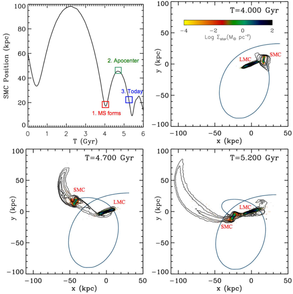
Fig. 1.— The orbit of the SMC about the LMC (without the MW). Top left: The separation between the Clouds as a function of time. The chosen orbit is highly eccentric ( e=0.7 ) and decays rapidly owing to dynamical friction. The Stream forms at 4 Gyr (red box) and the time today would correspond to \sim 5.2 Gyr (blue box). Subsequent Panels: The HI gas column density is plotted as contours over the stellar distribution for specific points in the orbit. Gas contours span a range of 10^{18} - 10^{20} /\text{cm}^2 , where each contour represents an increase in column density by a factor of 1.5. HI gas is identified as gas at temperatures below 12000 K and column densities larger than 10^{18} /\text{cm}^2 , although a background ionizing field is not included. A bridge of gas connecting the Clouds and a 100 kpc long gaseous stream with no stellar counterpart is formed without the aid of MW tides or ram pressure.
