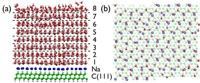
FIG. 1. (Color online) Visualization of epitaxial ice bilayers on the modified diamond surface. (a) Side view, showing the slab representing the C(111)-Na substrate at the bottom and the eight initially distinct bilayers of ice separated by dashed lines in an instantaneous configuration after 5 ps at 310 K. The distance between dashed lines is 3.7 Å. (b) Top view of bilayer 1 with C(111)-Na surface in background.
