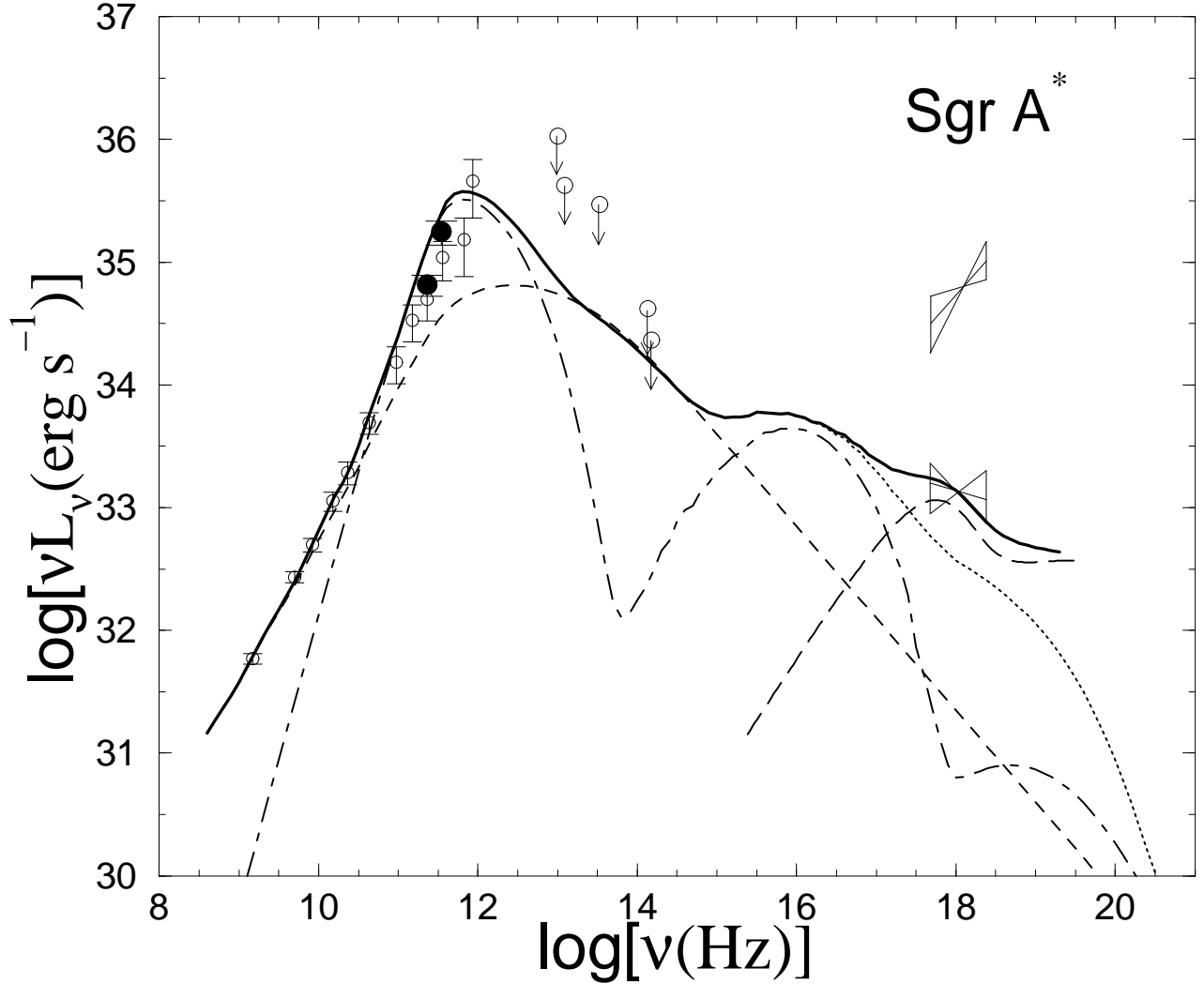
Fig. 1.— A model for the quiescent emission from Sgr A* with s = 0.27 , \delta = 0.55 . The accretion rate close to the BH is \dot{M} \approx 4 \times 10^{-8} M_\odot \text{ yr}^{-1} . The dot-dashed line is the synchrotron and IC emission by thermal electrons. The dashed line is the synchrotron emission by non-thermal electrons; the non-thermal electrons have \approx 1.5\% of the thermal energy with p = 3.5 . The dotted line is the total synchrotron and IC emission while the solid line includes the bremsstrahlung emission from the outer parts of the RIAF (shown by the long-dashed line); the latter component explains the extended quiescent X-ray source. The radio data are from Falcke et al. 1998 (open circles) and Zhao et al. 2003 (SMA; filled circles), the IR data are from Serabyn et al. (1997) and Hornstein et al. (2002). The two “bowties” in the X-ray are the quiescent (lower) and flaring (higher) data from Baganoff et al. (2001; 2003).
