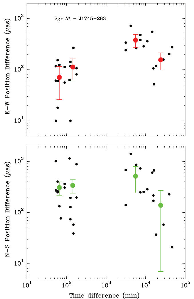
FIG. 2.— Position wander of Sgr A*. Plotted are east-west (top) and north-south (bottom) position differences as a function of time separation. Also shown are binned average position differences as large points with error bars. These position differences are likely caused by uncompensated atmospheric path delay errors and should be considered as upper limits to the position wander of Sgr A*.
