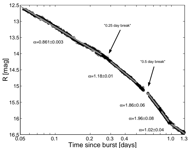
FIG. 9.— A detailed view of the early light curve of the OT associated with GRB 030329. The light curve distinctly breaks around 0.25 and 0.5 days. The data obtained prior to 0.25 days is not well described by a smooth power law, and shows significant wiggles. Note that our data rule out further steepening of the light curve at day 0.8, with the slope measured during 0.82 – 0.95 days consistent with the slope measured from earlier data (0.6 – 0.78 days) and certainly below the values \alpha \sim 2.2 reported elsewhere (see text). Around day 1 the decline in the optical flux begins to slow, as the rising branch of bump A emerges.
