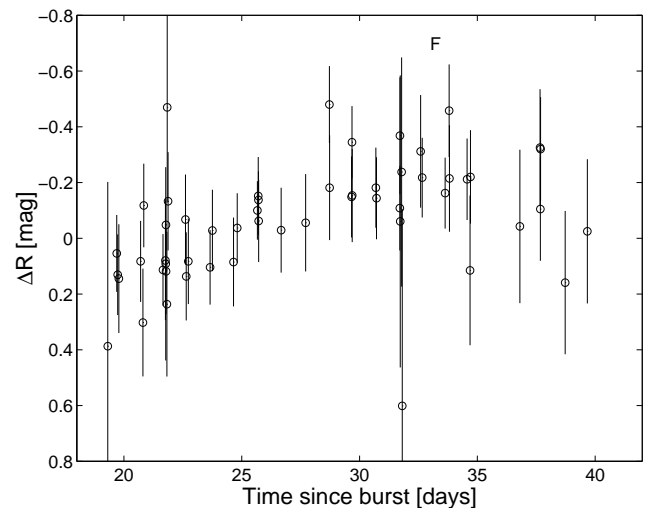
FIG. 7.— The variations light curve of the afterglow between day 18 and day 42.
