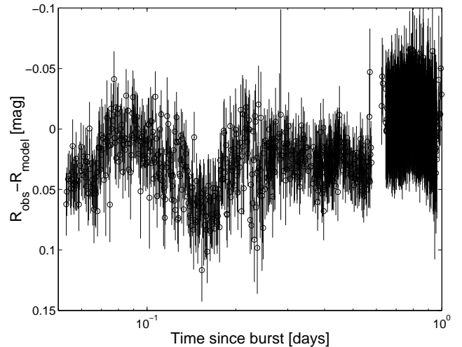
FIG. 12.— Same as Fig. 11, but zooming in on the period prior to the emergence of bump A . The residual undulations after subtraction of the Berger et al. (2003) two-jet model light curve are clearly evident.
