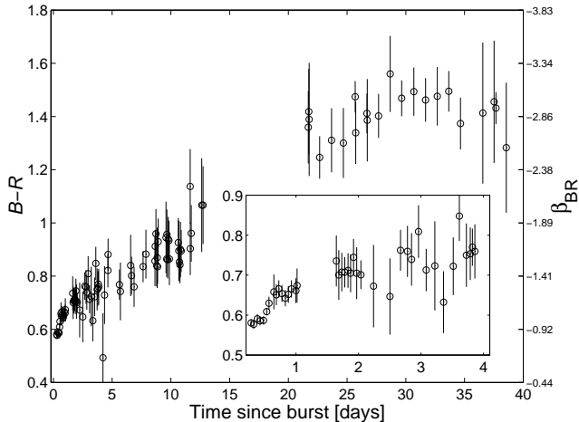
FIG. 8.— The binned (B - R) color of the OT during the first 40 days after the burst. The vertical axis on the right shows the corresponding spectral power-law, \beta_{BR} . The inset is a blow-up of the first four days.
