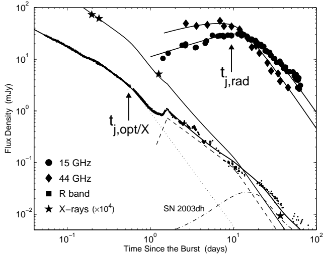
FIG. 10.— A comparison of the updated two-jet model with multi-band data. The model and notation are similar to those presented by Berger et al. (2003), except for several minor modifications (see text). The various symbols denote data points, as labeled, and the solid curves are the model predictions in each respective band. The model R -band light curve describes the general trends in the observed light curve well, but some discrepancies remain – the model becomes too bright around 10 days after the burst, and later on becomes too faint.
