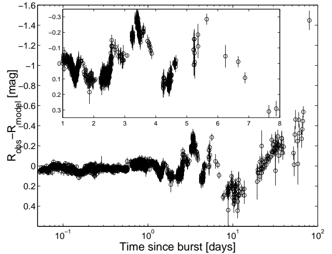
FIG. 11.— The residual light curve obtained by subtracting the modified two-jet model from the observed R -band light curve. Note that at t \leq 1 day the model describes the general light curve trends very well, but significant wiggles around the smooth trend remain. A phase of strong variations can be seen between 1 – 8 days, followed by broader undulation around the predicted peak of SN 2003dh, that may be associated with inadequacies in the SN model. During later times ( \gtrsim 20 days), the data seem to require yet another source of optical emission, which is also strongly variable. The inset is a magnified view of the strong variations between, day 1 and day 8
