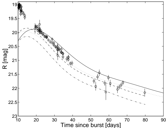
FIG. 2.— The host-subtracted R -band light curve of the OT (open circles) compared to four model light curves of SN 2003dh. The plotted lines are: the light curve of SN 1998bw, redshifted and K -corrected (solid line); the same model, after applying the best fitting magnitude shift and temporal shift relative to the GRB (see text; dotted line); the same model, after applying the best fitting magnitude-shift and stretch correction (see text; dashed line); and the time-stretched and magnitude-shifted model lowered by 0.3 mag (dash-dotted line).
