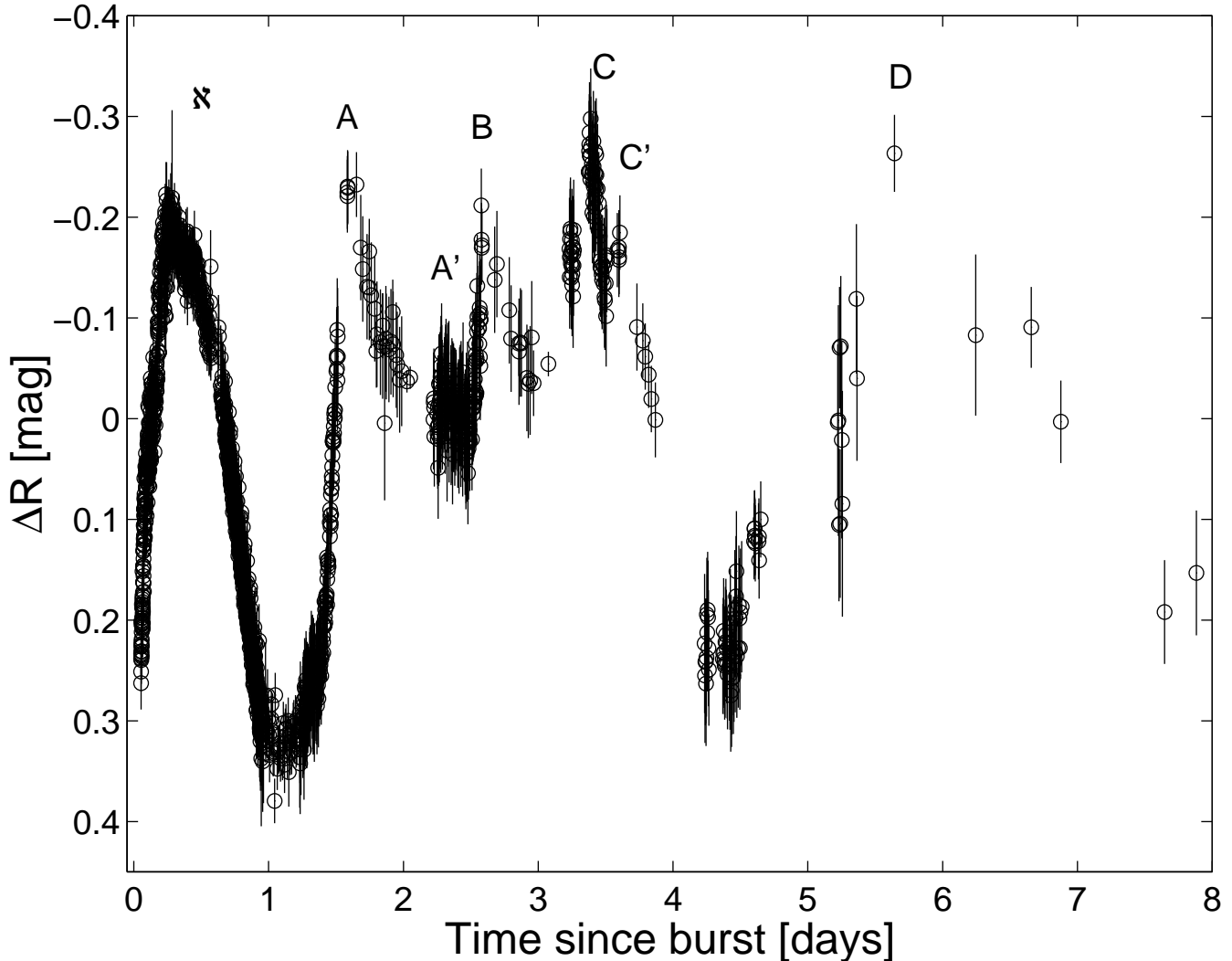
FIG. 4.— The residual light curve, obtained by subtracting our best fit double power-law (see text) from the light curve of the afterglow, during the first eight days after the burst. Five strong bumps, along with two possible minor ones, are apparent in the light curve.
