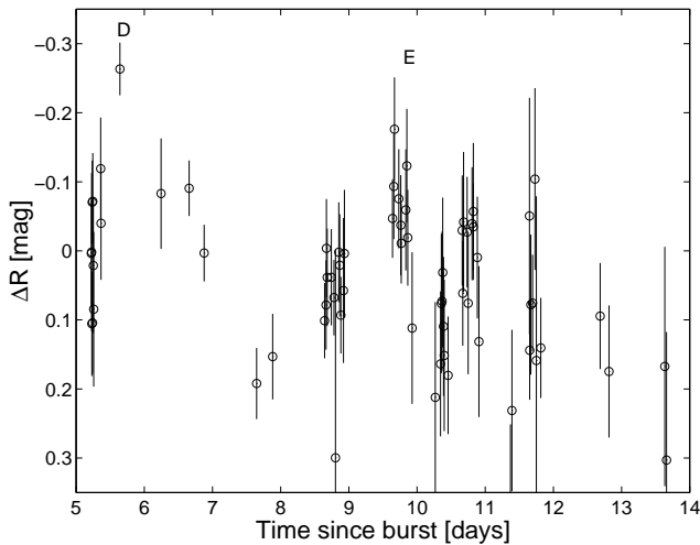
FIG. 6.— The variations light curve of the afterglow between day 5 and day 14.
