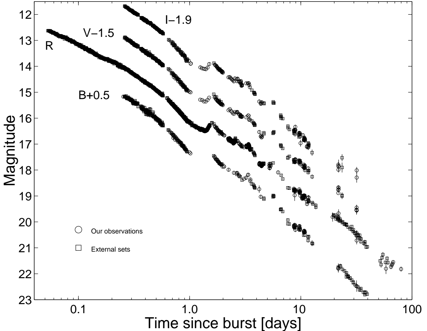
FIG. 1.— BVR light curve of GRB 030329. Our observations are marked by circles, and the external data sets (see Table 1), cross-calibrated to our photometric system, are marked by squares. For presentation purposes the BVI light curves are shifted vertically by +0.5, -1.5, and -1.9 mag, respectively.
