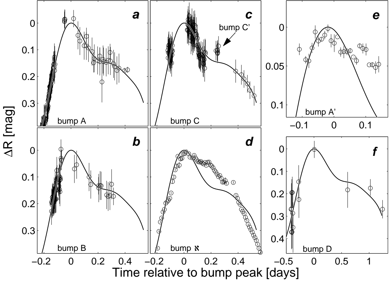
FIG. 5.— A close up view of the main bumps detected in the early residual light curve, which was obtained by subtracting our best fit double power-law (see text) from the light curve of the afterglow. Panels a , b , c , d , e , and f , display bumps A, B, C, X, A', and D, respectively. The light curves in panels d and e were binned, to allow convenient browsing. The solid curves are a smoothed fit to the superimposed light curves of bumps A, B, and C, representing the common structure of these three bumps (see text for details). The time scale of the curve in panel f was stretched by a factor of 2.3.
