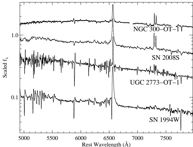
Figure 5. Optical spectra of UGC 2773 OT2009-1, NGC 300 OT2008-1 (Berger et al. 2009b), SN 1994W (Chugai et al. 2004), and SN 2008S (Smith et al. 2008b). All spectra have narrow H \alpha and [Ca II] emission; however, NGC 300 OT2008-1 and SN 2008S lack the forest of lines (especially Fe II) that UGC 2773 OT2009-1 and SN 1994W display.
