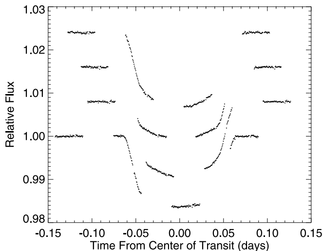
FIG. 1.—Normalized time series spanning the entire wavelength range of the grating for the four transits observed. Transits occurred (from top to bottom) on UT 2003 May 3 (HJD 2452763.7, G430L grating), May 31 (HJD 2452791.4, G750L grating), June 25 (HJD 2452816.1, G430L grating), and July 5 (HJD 2452826.6, G750L grating). Each successive transit is offset by 0.008 in relative flux.
