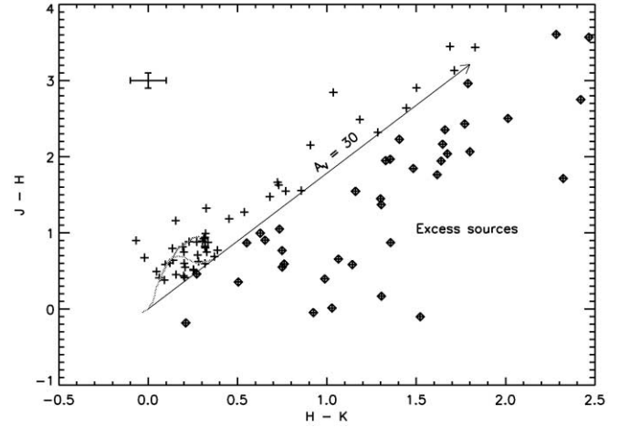
FIG. 11.— J-H vs. H-K_S plot of 2MASS sources matched with ChaMPlane sources in this paper. Overlaid is the locus of dwarf and giant stars (giant stars are redder) from Bessell & Brett (1988). The arrow represents an extinction of A_V = 30 using the extinction relation of Nishiyama et al. (2006). Sources marked with diamond points are candidate excess sources/young stars. A typical error bar is shown in the upper left.
