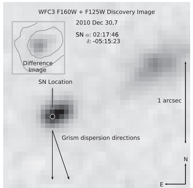
Figure 1. The WFC3 F160W + F125W discovery and difference images (using a late-time, SN-free template) for SN UDS10Wil. The SN is located \sim 0.1 from the center of the host galaxy (2 ACS pixels). The contours plotted on the difference image of the SN (upper left) show the regions containing 68% and 95% of the host galaxy light. The center of the nearest neighboring galaxy, which causes minimal lensing of the SN (see Section 4.1), is located \sim 1.5 away.
