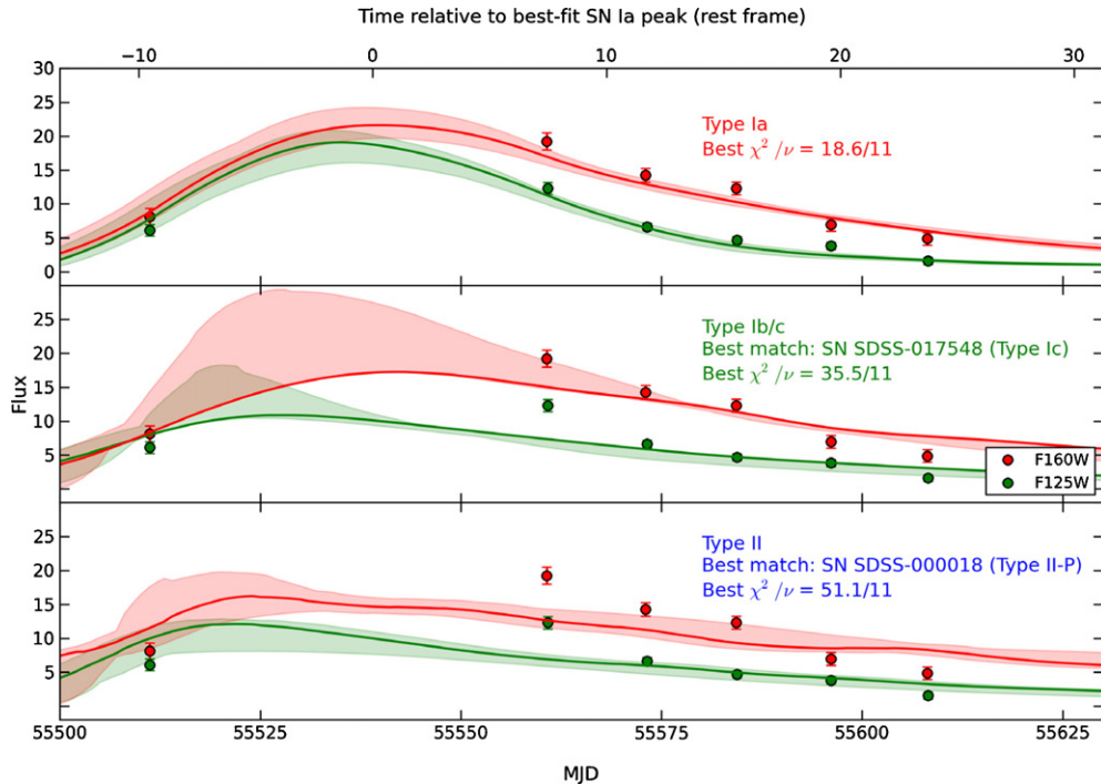
Figure 2. The best-fit light curves using SNANA-simulated Type Ia, Type Ib/c, and Type II SNe (top to bottom). Red and green colors indicate photometry and simulations for the F160W and F125W filters (approximately rest-frame B and V ), respectively. Shaded regions include the range of SN fits that encompass 95% of the Bayesian evidence for a given SN type. Type Ib/c and Type II fits have higher \chi^2 values (even including model uncertainties), due to their inability to match the combination of the colors nearest to maximum light and the rapid rate of decline. The sum of the evidence for a SN Ia model gives a nearly 100% probability that the SN is of Type Ia. We included F814W and F850LP data in the \chi^2 fitting, but have omitted them in this figure for visual clarity. The fluxes shown are transformed from Vega magnitudes using a zero point of 27.5.
