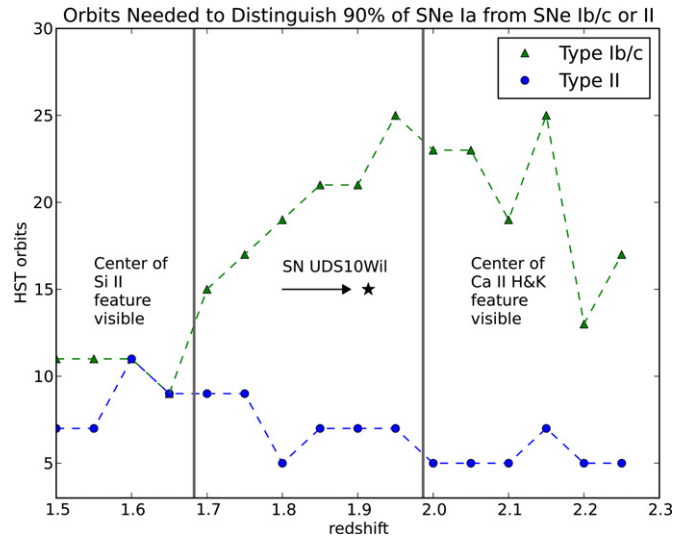
Figure 5. The number of orbits necessary to rule out the possibility of a SN II or SN Ib/c 90% of the time when observing a SN Ia. Using aXeSim, we simulated a variety of exposure times in the redshift range 1.5–2.3. We found that \sim 5\text{--}10 orbits can rule out a SN II, but that the number of orbits required to rule out a SN Ib/c possibility is significantly greater. The number of orbits to rule out a SN Ib/c is much lower in the region where Si II and Ca II H&K are completely visible. These results indicate the need for photometric evidence in SN Ia classification at high redshift, although the HST grism can also be valuable in determining SN redshifts.
