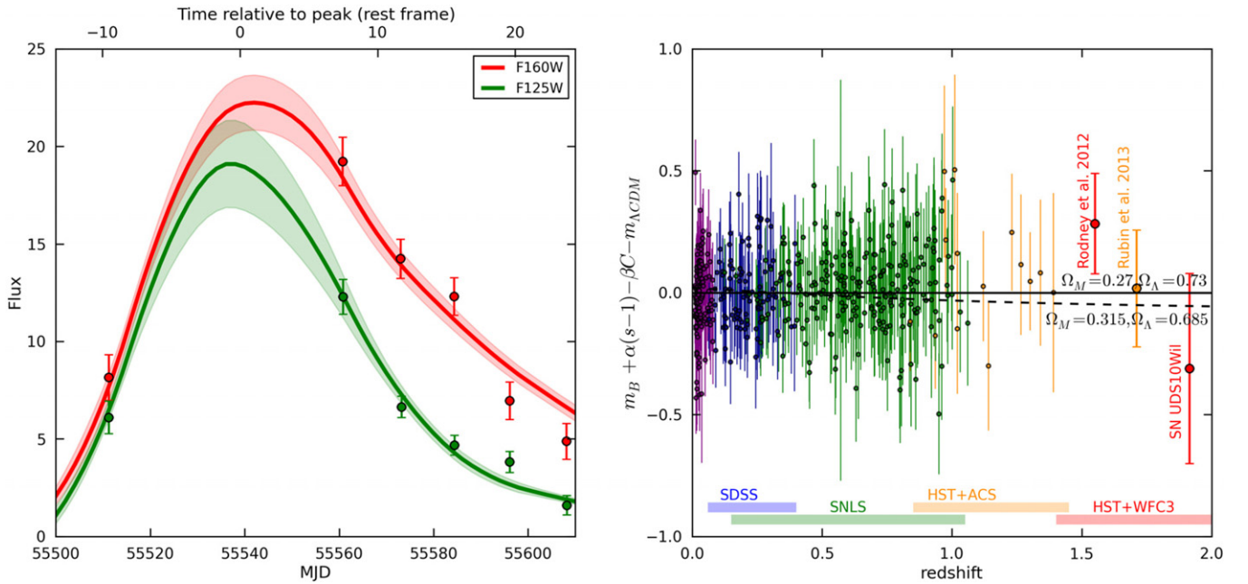
Figure 4. On the left, the SALT2 light-curve fit to SN UDS10Wil. SALT2 gives a normal set of light-curve parameters along with a corrected magnitude of 26.15 \pm 0.39 (consistent with \Lambda CDM) and a reduced \chi^2 of 1.5. On the right, we place SN UDS10Wil on the Hubble residual diagram using cosmological parameters from Sullivan et al. (2011) and H_0 = 71.6 \text{ km s}^{-1} \text{ Mpc}^{-1} . For comparison, we also show the compilation of \sim 500 SNe from Conley et al. (2011). Lastly, using Sullivan et al. (2011) values for \alpha and \beta , we include the other two SNe Ia with spectroscopic evidence for classification discovered at a redshift greater than 1.5 (Rodney et al. 2012; Rubin et al. 2013). The dotted line indicates the difference in m_{\Lambda\text{CDM}} when using the recent cosmological parameters from the Planck collaboration ( \Omega_{\Lambda} = 0.685 , \Omega_M = 0.315 ; Planck Collaboration et al. 2013).
