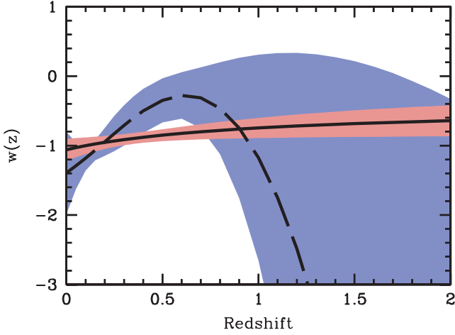
FIG. 11.—Best solution and uncertainty for a quartic polynomial fit (blue), and simple w_0-w_a parameterization using a strong prior (red). As seen, the simple parameterization highly constrains the behavior of w(z) as compared to the polynomial. The greater constraint on w(z) implied by the w_0-w_a parameterization derives from implicit and unjustified priors on dark energy: that its evolution is monotonic, linear, and most important at low redshifts.
