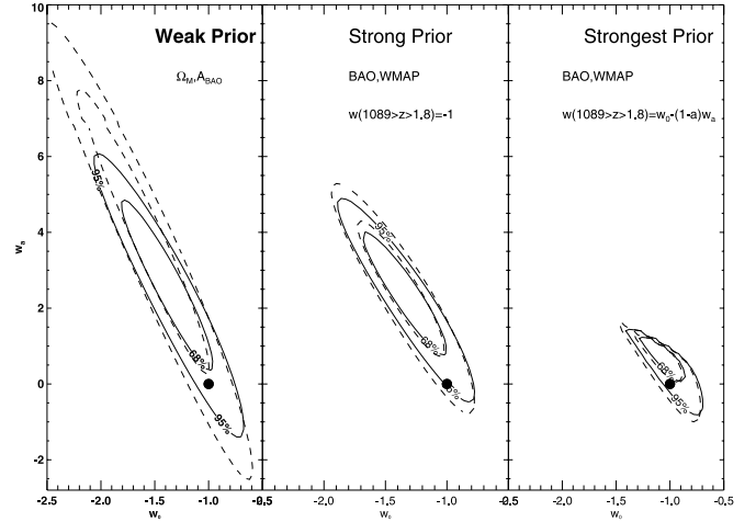
FIG. 10.— Joint confidence intervals derived from SN samples for a two-parameter model of the equation-of-state parameter of dark energy, w(z) = w_0 + w_a z / (1+z) . For each panel, constraints from a SN sample are combined with the indicated prior to yield the indicated confidence intervals. The position of a cosmological constant (-1, 0) is shown as a filled symbol.
