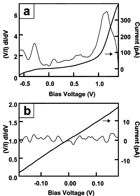
FIG. 4. (a) Low resolution and (b) high resolution I - V and normalized conductance data recorded on a MoSe wire at 5 K; the substrate was Au(111). The high-resolution data was recorded after advancing the tip closer to the wire to improve the signal to noise in the current. The variation in (V/I)dI/dV in (b) corresponds to noise.
