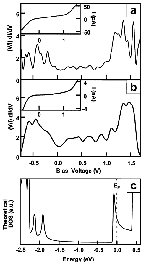
FIG. 3. I - V data (inset) and normalized conductance of MoSe wires deposited on (a) Au(111) and (b) HOPG. The features in (b) are not as sharp as in (a) but the positions of the peaks are the same. The data in (a) and (b) were recorded at 298 K. The approach of (V/I)dI/dV to 0 at voltage limits in (b) is an artifact of the data treatment. (c) Density of states (DOS) calculated from the band structure of [13,16] showing a 1.8 eV separation between the first VHS arising from bonding and antibonding d bands.
