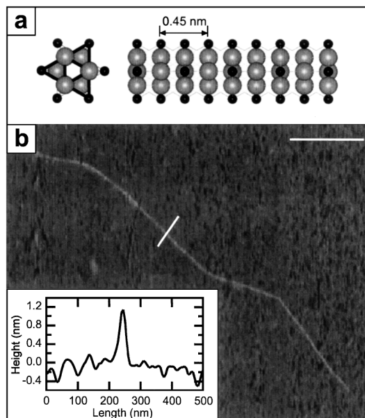
FIG. 1. (a) Structural model of a \text{Mo}_6\text{Se}_6 ( \text{MoSe} ) molecular wire based on the \text{Li}_2\text{Mo}_6\text{Se}_6 crystal structure [9,10]. (b) Tapping mode atomic force microscopy (AFM) image of a \text{MoSe} wire deposited on a cleaved mica surface from methanol solution. The white scale bar corresponds to 1 \mu\text{m} . Inset: Section across the sample at the position of the white line. The width of the section is much larger than the height due to the convolution of the AFM tip.
