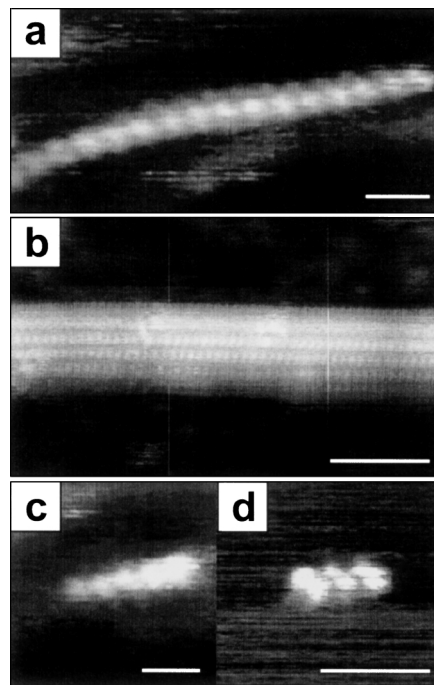
FIG. 2. STM height images, obtained in constant current mode, of MoSe chains deposited from methanol or acetonitrile solutions of \text{Li}_2\text{Mo}_6\text{Se}_6 on an Au(111) substrate at 298 K. (a) A single chain imaged at a sample bias of 0.8 V and a tunneling current of 50 pA (scale bar is 1 nm), and (b) a MoSe wire bundle imaged at a sample bias of 0.75 V and a tunneling current of 50 pA (scale bar is 5 nm). (c) and (d) Images of MoSe wire fragments containing 5 (0.8 V, 50 pA) and 3 (0.5 V, 150 pA) unit cells, respectively; the scale bars are 1 nm.
