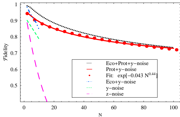
FIG. 4: (Color Online) Fidelity to create GHZ state as a function of N for systems in the presence of \sigma_y noise : without MPM (green dashed line), without MPM but with spin echo (dot-dashed blue line), with MPM (red solid line) and with both MPM and echo (dotted black line). We also show the degradation caused by pure dephasing in an unprotected system (long dashed purple line) for comparison purposes. For simplicity we assumed infinite correlation time: f(\omega) = \Upsilon \delta(\omega/\chi) , \Upsilon = 0.1\chi . The echo technique consisted of a perfect sudden \pi pulse around the x direction at \chi t = \pi/4 . Because the y components of the noise do not commute with \hat{J}_z^{(0)} the dynamics was solved numerically. For the unprotected system all the 2^N states had to be considered and we had to limit the particle number by N = 10 . On the other hand the restriction of the dynamics to the MPM in the protected scheme allowed us to extend the calculation to larger N values. For the \sigma_y noise the fidelity with protection does not become N independent, but instead scales as e^{-0.043N^{0.44}} (see fitted red dots). Nevertheless we do gain a factor of order \sqrt{N} with respect to the unprotected system. The plot also shows that the combination of MPM with spin echo provides the best protection.
