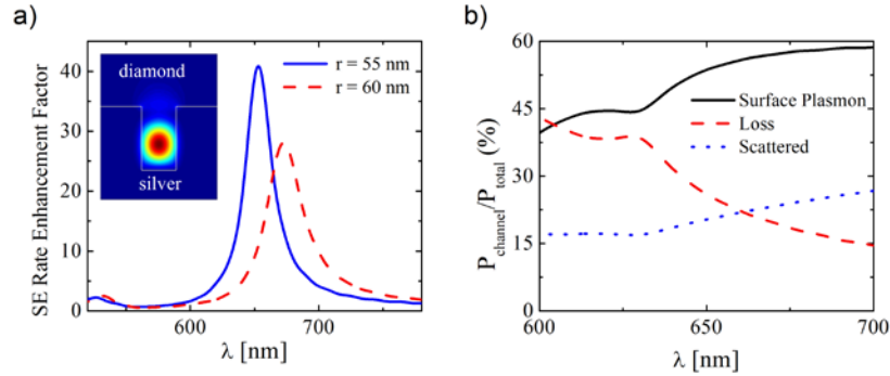
Fig. 6. (a) SE Rate enhancement spectrum of a dipole inside the plasmonic apertures. Inset: mode profile. (b) Coupling efficiency in to surface plasmons, non-radiative channels and radiation modes.
