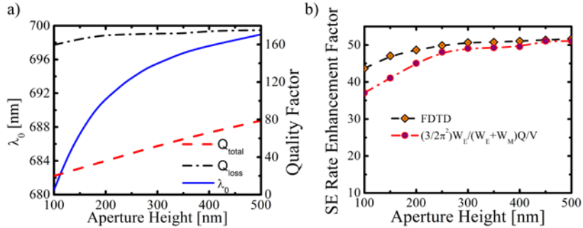
Fig. 4. (a) Resonant wavelengths and the corresponding quality factors as a function of aperture height for r = 50 nm. (b) SE rate enhancement factor from the modified Purcell formula and from FDTD as a function of height for r = 50 nm.
