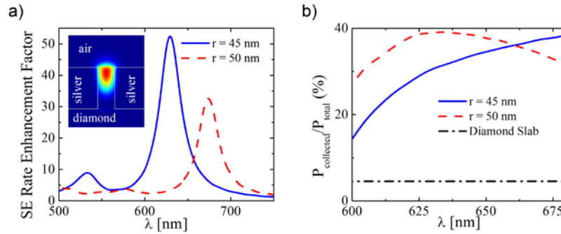
Fig. 5. (a) SE rate enhancement spectrum for r = 45 and 50 nm apertures. Inset: mode profile. (b) Total collection efficiency from a plasmonic aperture and a diamond slab when a lens with 0.95 N.A. is used.
