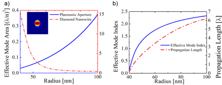
Fig. 2. (a) Mode area for the HE11 mode of a plasmonic aperture and a diamond nanowire at 637 nm. Inset: electric energy density distribution for the guided mode in the case of the aperture. (b) Effective mode index and propagation length in units of wavelength for plasmonic aperture.
