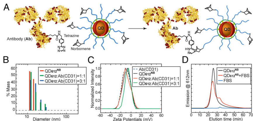
Fig. 1. QD NB-Tz Ab nanoconjugate synthesis and characterization. (A) Conjugation of QDs to Abs. Ab (IgG 2a ) is used to represent the Ab, and Lys residues of Ab(IgG 2a ) are marked in red. This diagram is not to scale. (B) Dynamic light scattering data of the QDs and the QD NB-Tz Ab illustrate that QD NB /Ab conjugation does not yield noticeable aggregates and that the size of QD NB-Tz Ab is compact. (C) \zeta -Potential measurements of the QDs and the QD NB-Tz Ab show that the surface charge of QD NB and QD NB-Tz Ab is moderately negative. (D) Gel filtration chromatography (GFC) traces of QD 612 NB before and after serum incubation show that there is virtually no nonspecific binding of QD NB to serum proteins.
