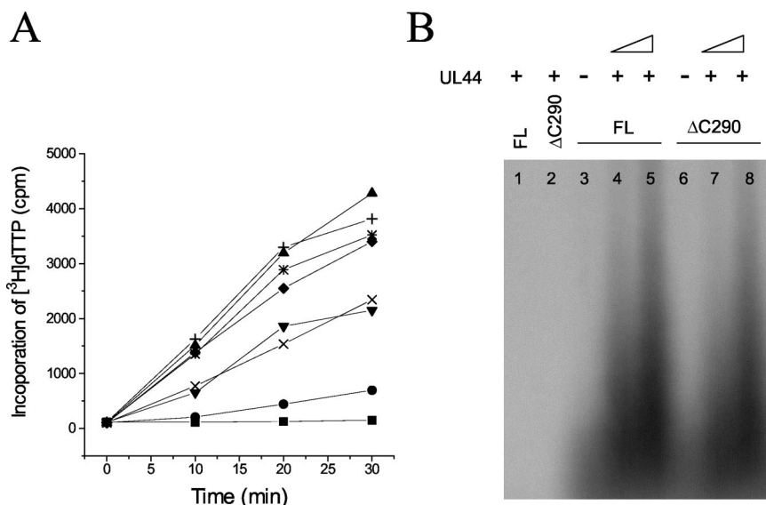
FIG. 4. UL44ΔC290 stimulates DNA synthesis by UL54. (A) The DNA polymerase activity of purified baculovirus-expressed UL54 alone (●) and in the presence of 200 (▼), 500 (*), or 1,000 (▲) fmol of GST-UL44 (full length) or of 200 (×), 500 (◆), or 1,000 (+) fmol of GST-UL44ΔC290 alone (■) was also assayed. Samples were taken after 0, 10, 20, and 30 min of incubation at 37°C and spotted onto DE81 filters. The filters were washed, and radioactivity was counted. (B) Stimulation of UL54-mediated long-chain DNA synthesis by GST-full-length UL44 (FL) or GST-UL44ΔC290 (ΔC290) was assayed by measuring the incorporation of labeled TTP on a poly(dA)-oligo(dT) DNA template. The reaction products were visualized by autoradiography following electrophoresis on a 4% alkaline agarose gel. Lane 1 contains 800 fmol of GST-UL44 (full-length) alone; lane 2 contains 800 fmol of GST-UL44ΔC290 alone; lanes 3 and 6 contain 200 fmol of UL54 alone; lanes 4 and 5 contain UL54 plus 400 and 800 fmol of GST-UL44 (full-length), respectively; lanes 7 and 8 contain UL54 plus 400 and 800 fmol of GST-UL44ΔC290, respectively.
