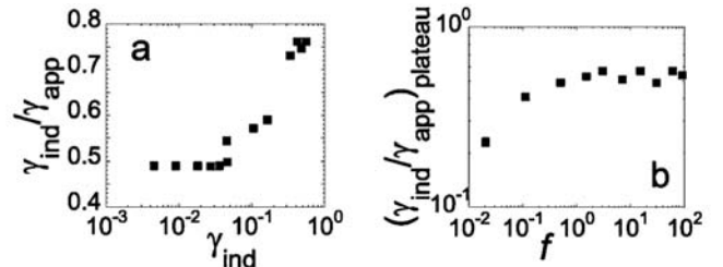
FIG. 3. (a) The ratio \gamma_{ind}/\gamma_{app} vs \gamma_{ind} for f = 60 Hz. (b) Plot of the \gamma_{ind}/\gamma_{app} low strain plateau vs f .
