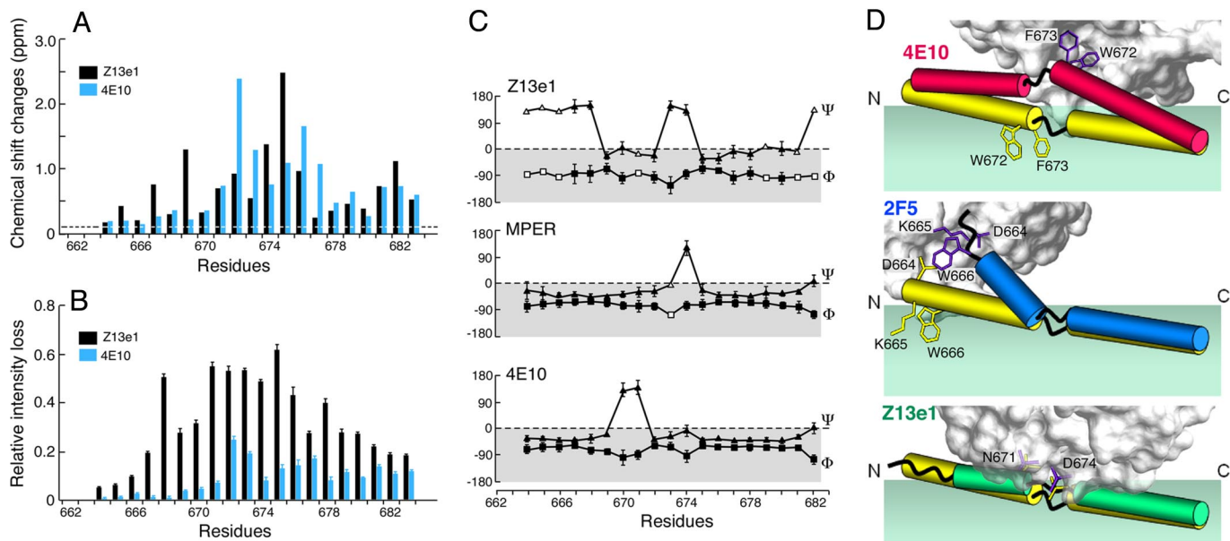
Fig. 2. Comparison of MPER conformational changes induced by Z13e1 and 4E10. (A) Normalized amide chemical shift changes \{[\Delta(\text{Hcs})^2 + (\Delta\text{Ncs}/5)^2]^{1/2}\} of Z13e1 Fab-bound (black) and 4E10 Fab-bound (blue) MPERs relative to the unbound peptide in DPC micelles. Indicative chemical shift change (0.1 ppm) is shown with a dotted line. (B) MPER residues involved in Z13e1 (black) and 4E10 (blue) interactions shown by NMR cross-saturation transfer are indicated by relative signal reduction of amide peaks after 250-ms irradiation in methyl region. Cross-saturation transfer efficiencies are higher in Z13e1-bound MPERs because of higher immobility induced by tight Fab binding. The error bars represent statistical errors resulting from uncertainties in peak integration. (C) Comparison of backbone dihedral angles of the MPER in the absence ( Middle ) and presence of Z13e1 ( Top ) and 4E10 ( Bottom ), predicted from chemical shift values of \text{C}\alpha/\text{C}\beta . The \Phi and \Psi angles are shown in square and triangle symbols, respectively (symbols in white correspond to statistically less reliable predictions). (D) Artistic rendering of MPER orientation changes induced by 4E10, 2F5, and Z13e1. Unbound MPER peptides (yellow tubes) are immersed in the lipid bilayers (light green panel). Red, blue, and green tubes represent the membrane orientation of schematic MPER segments in complex with 4E10, 2F5, and Z13e1 (gray surface area), respectively. N and C termini of MPER peptides are marked by letters N and C, respectively. Several key binding residues' positions are indicated before (yellow) and after (purple) antibody binding. For simplicity, the exact 3-dimensional features of MPER segments and Fabs are not visualized here. (See Fig. S9 for examples of structural details.)
